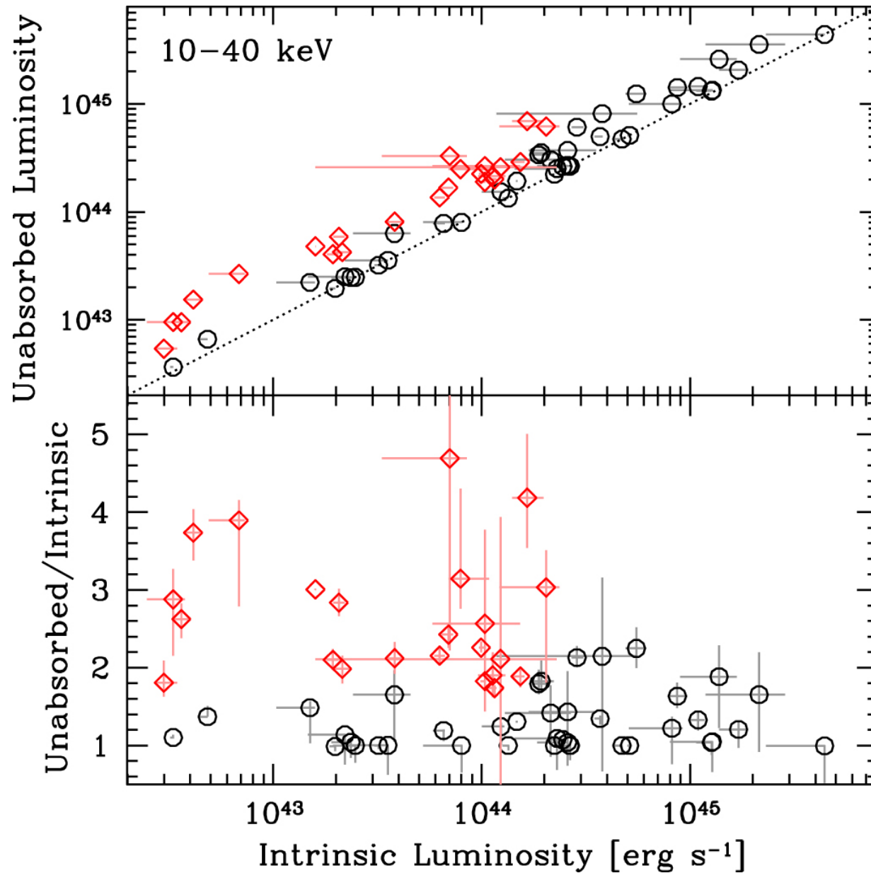
Figure 6. from The NuSTAR Extragalactic Surveys: X-Ray Spectroscopic Analysis of the Bright Hard-band Selected Sample null 2018 APJ 854 33 doi:10.3847/1538-4357/aaa550 https://dx.doi.org/10.3847/1538-4357/aaa550 © 2018. The American Astronomical Society. All rights reserved.
