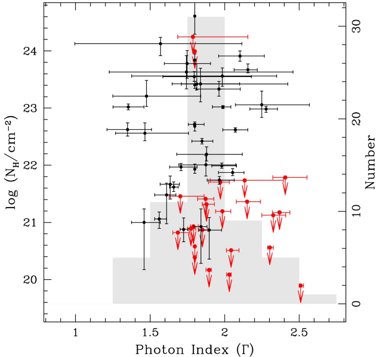
Figure 5. from The NuSTAR Extragalactic Surveys: X-Ray Spectroscopic Analysis of the Bright Hard-band Selected Sample null 2018 APJ 854 33 doi:10.3847/1538-4357/aaa550 https://dx.doi.org/10.3847/1538-4357/aaa550 © 2018. The American Astronomical Society. All rights reserved.
