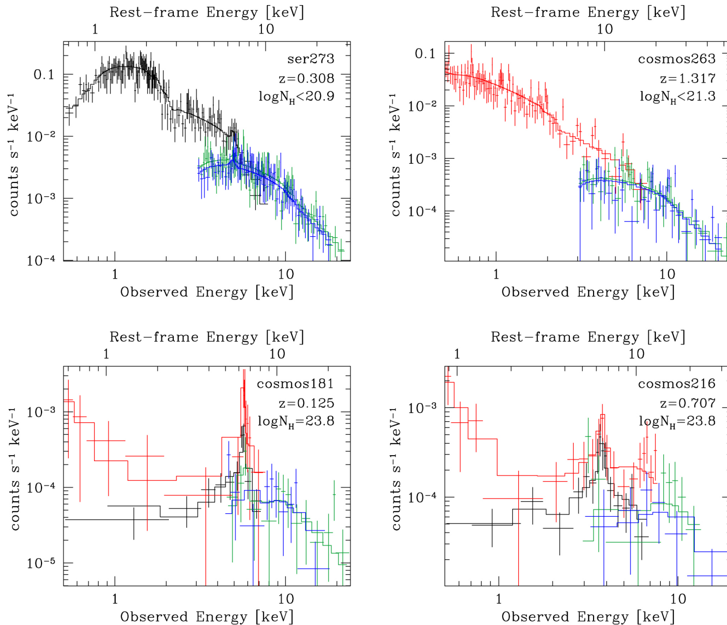
Figure 4. from The NuSTAR Extragalactic Surveys: X-Ray Spectroscopic Analysis of the Bright Hard-band Selected Sample null 2018 APJ 854 33 doi:10.3847/1538-4357/aaa550 https://dx.doi.org/10.3847/1538-4357/aaa550 © 2018. The American Astronomical Society. All rights reserved.
