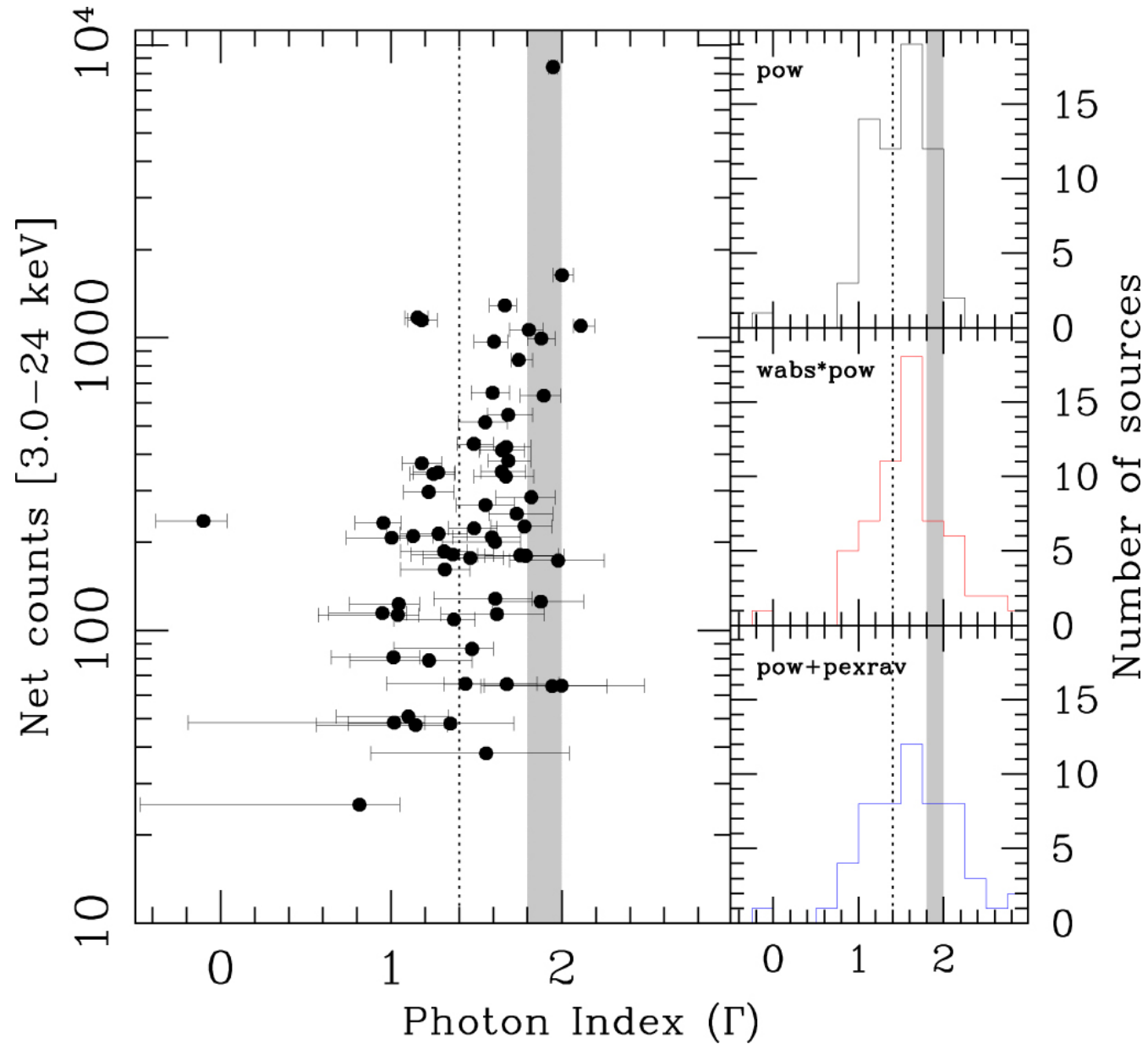
Figure 3. from The NuSTAR Extragalactic Surveys: X-Ray Spectroscopic Analysis of the Bright Hard-band Selected Sample null 2018 APJ 854 33 doi:10.3847/1538-4357/aaa550 https://dx.doi.org/10.3847/1538-4357/aaa550 © 2018. The American Astronomical Society. All rights reserved.
