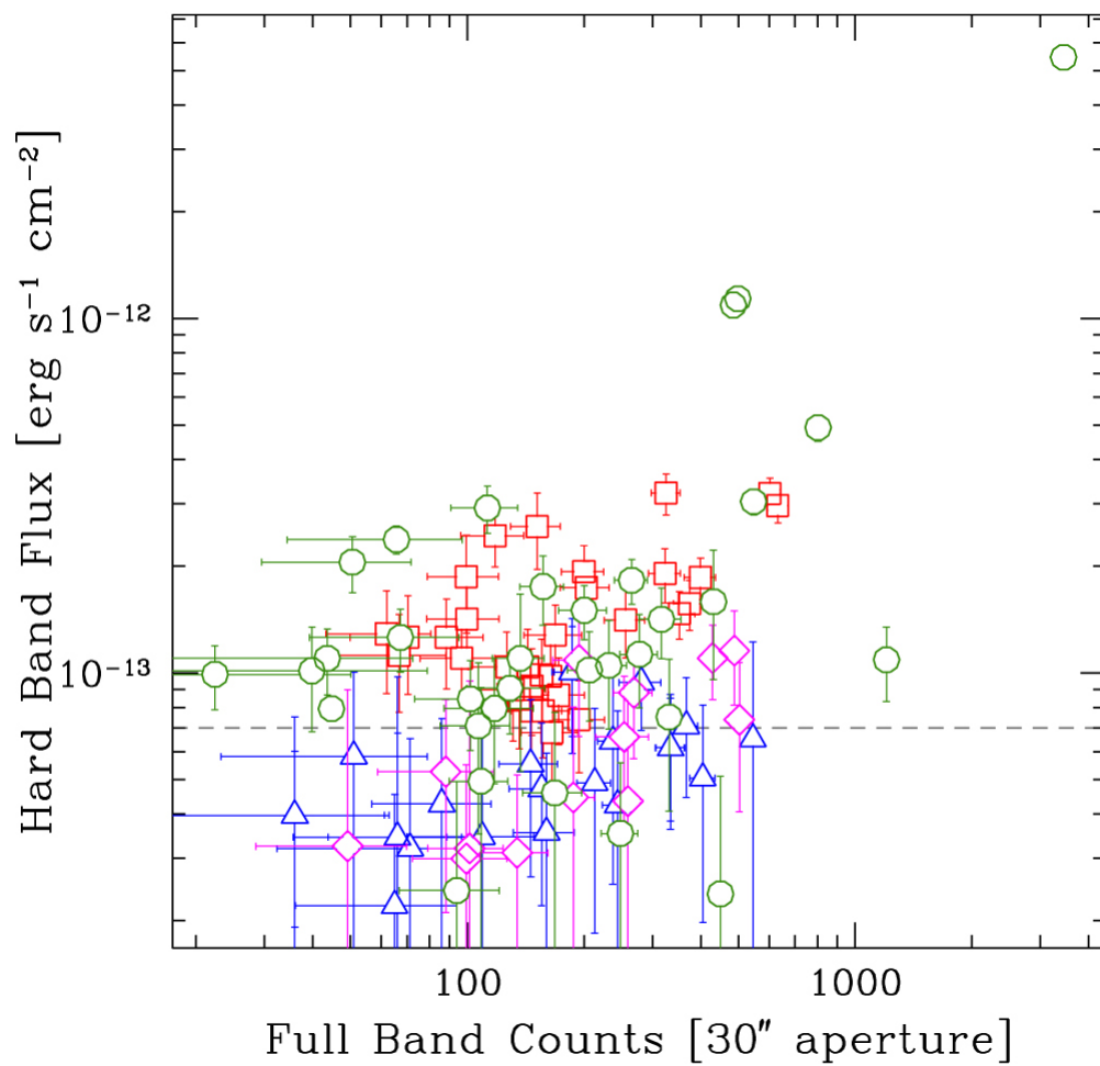
Figure 2. from The NuSTAR Extragalactic Surveys: X-Ray Spectroscopic Analysis of the Bright Hard-band Selected Sample null 2018 APJ 854 33 doi:10.3847/1538-4357/aaa550 https://dx.doi.org/10.3847/1538-4357/aaa550 © 2018. The American Astronomical Society. All rights reserved.
