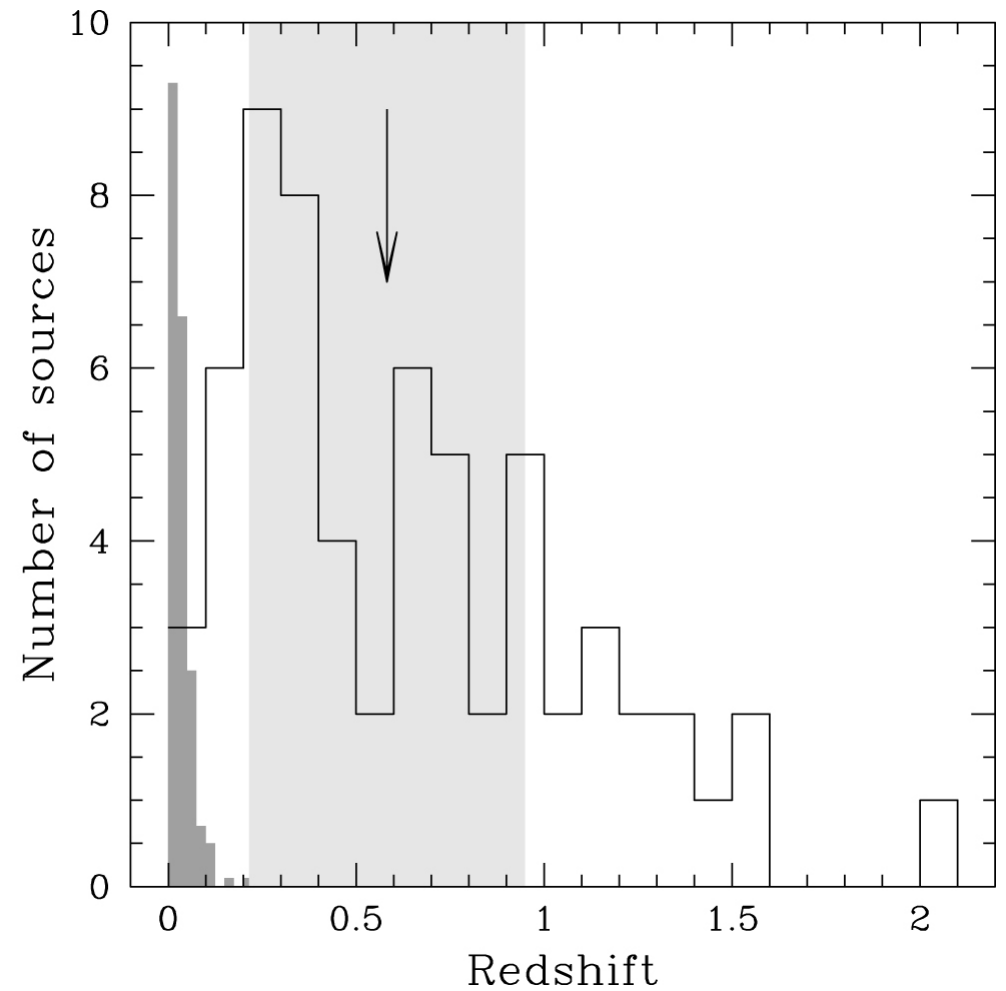
Figure 2. from The NuSTAR Extragalactic Surveys: X-Ray Spectroscopic Analysis of the Bright Hard-band Selected Sample null 2018 APJ 854 33 doi:10.3847/1538-4357/aaa550 https://dx.doi.org/10.3847/1538-4357/aaa550 © 2018. The American Astronomical Society. All rights reserved.
