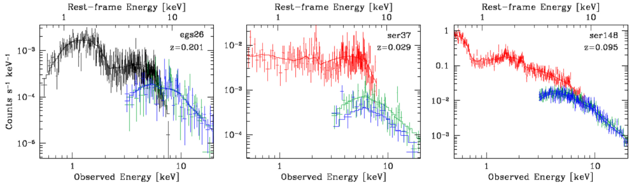
Figure 17. from The NuSTAR Extragalactic Surveys: X-Ray Spectroscopic Analysis of the Bright Hard-band Selected Sample null 2018 APJ 854 33 doi:10.3847/1538-4357/aaa550 https://dx.doi.org/10.3847/1538-4357/aaa550 © 2018. The American Astronomical Society. All rights reserved.
