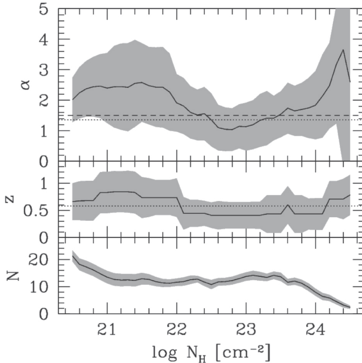
Figure 15. from The NuSTAR Extragalactic Surveys: X-Ray Spectroscopic Analysis of the Bright Hard-band Selected Sample null 2018 APJ 854 33 doi:10.3847/1538-4357/aaa550 https://dx.doi.org/10.3847/1538-4357/aaa550 © 2018. The American Astronomical Society. All rights reserved.
