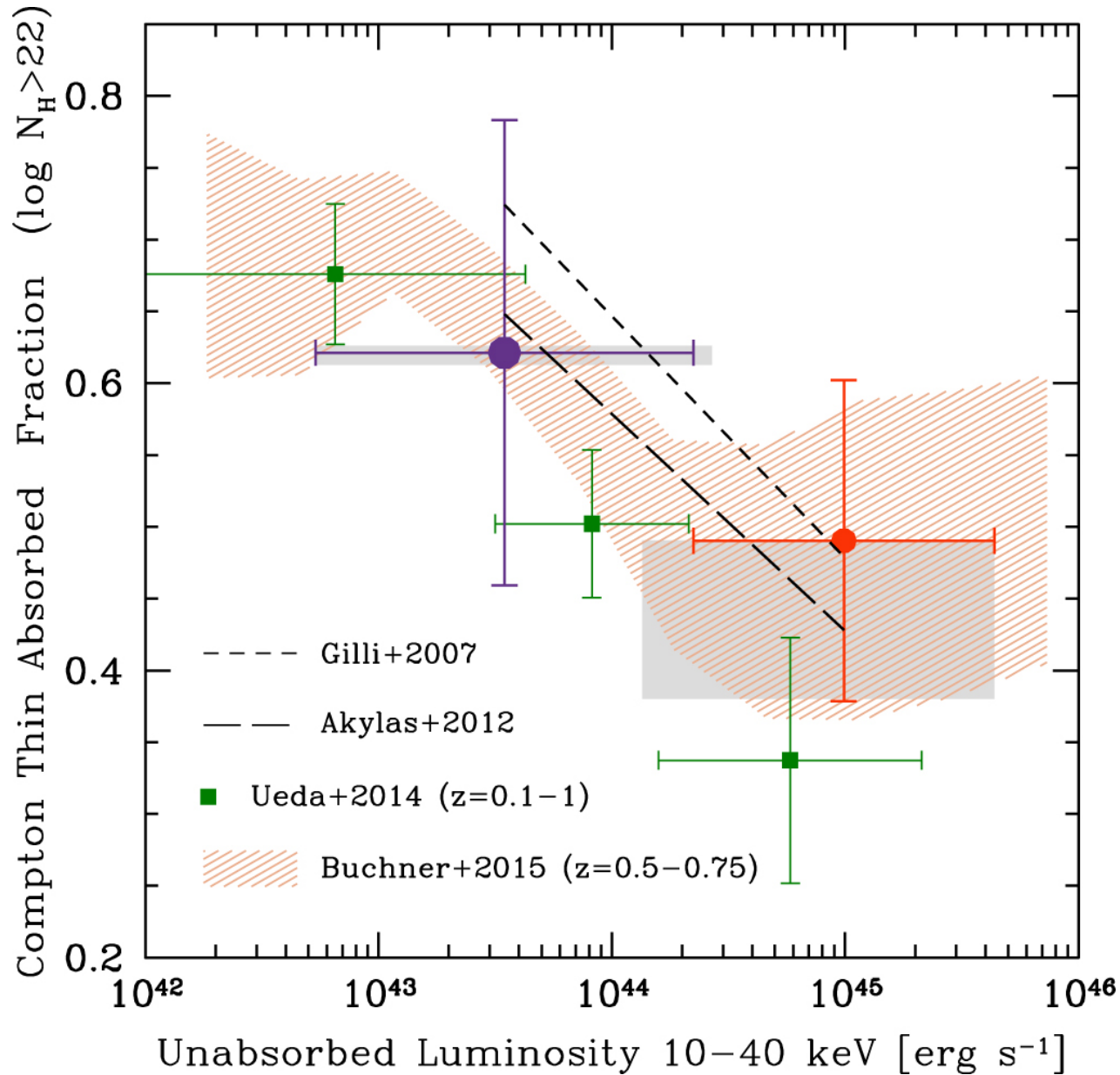
Figure 13. from The NuSTAR Extragalactic Surveys: X-Ray Spectroscopic Analysis of the Bright Hard-band Selected Sample null 2018 APJ 854 33 doi:10.3847/1538-4357/aaa550 https://dx.doi.org/10.3847/1538-4357/aaa550 © 2018. The American Astronomical Society. All rights reserved.
