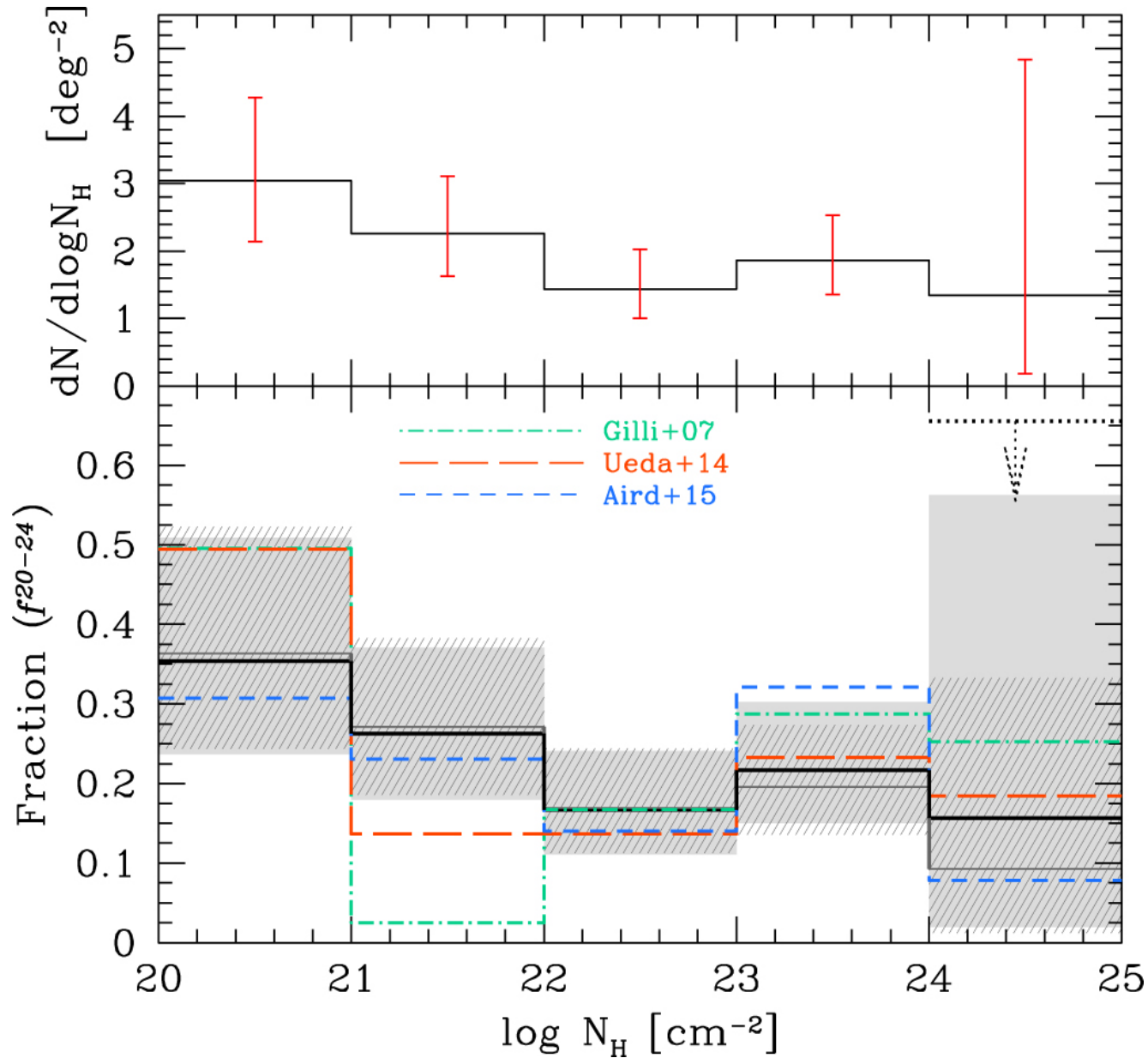
Figure 12. from The NuSTAR Extragalactic Surveys: X-Ray Spectroscopic Analysis of the Bright Hard-band Selected Sample null 2018 APJ 854 33 doi:10.3847/1538-4357/aaa550 https://dx.doi.org/10.3847/1538-4357/aaa550 © 2018. The American Astronomical Society. All rights reserved.
