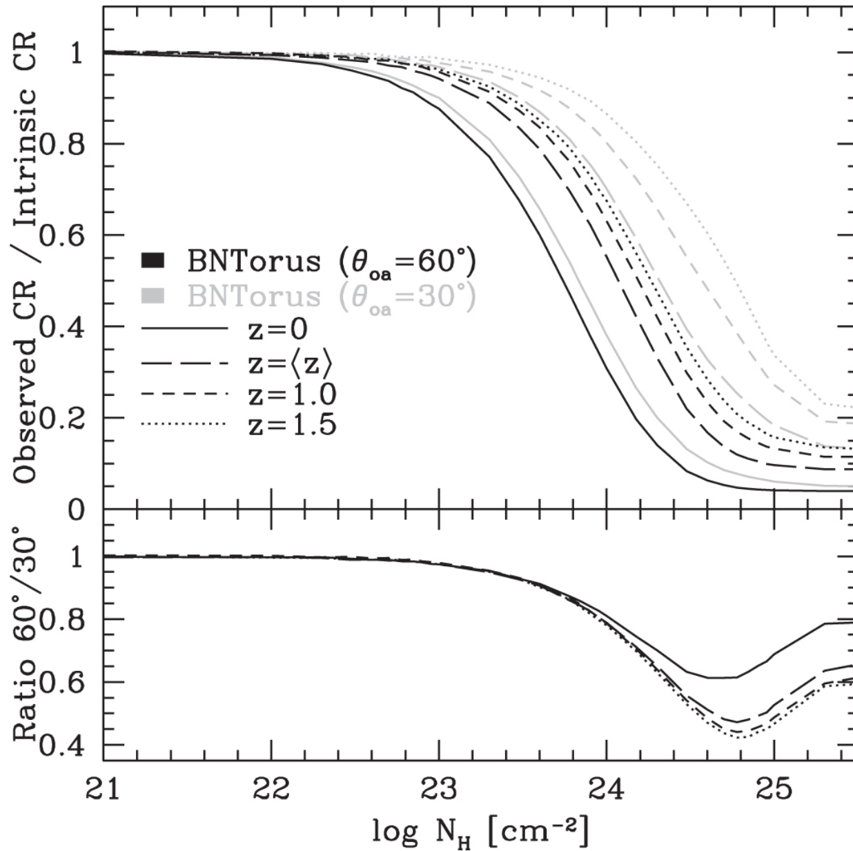
Figure 11. from The NuSTAR Extragalactic Surveys: X-Ray Spectroscopic Analysis of the Bright Hard-band Selected Sample null 2018 APJ 854 33 doi:10.3847/1538-4357/aaa550 https://dx.doi.org/10.3847/1538-4357/aaa550 © 2018. The American Astronomical Society. All rights reserved.
