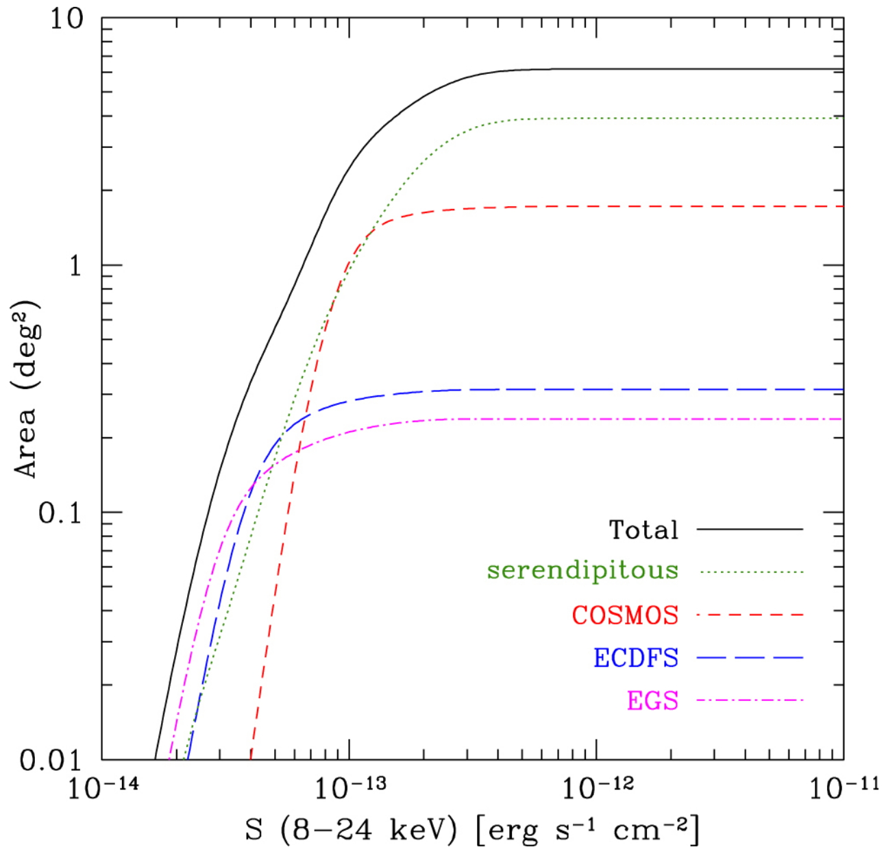
Figure 1. from The NuSTAR Extragalactic Surveys: X-Ray Spectroscopic Analysis of the Bright Hard-band Selected Sample null 2018 APJ 854 33 doi:10.3847/1538-4357/aaa550 https://dx.doi.org/10.3847/1538-4357/aaa550 © 2018. The American Astronomical Society. All rights reserved.
