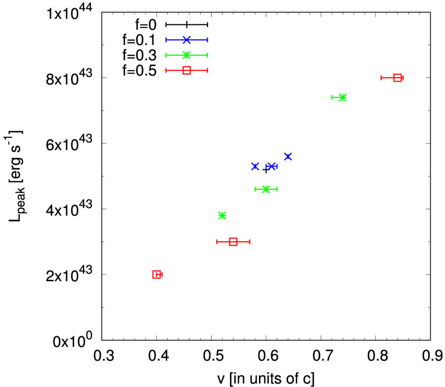
Figure 8. from X-Ray Light Curve and Spectra of Shock Breakout in a Wind null 2018 APJ 853 52 doi:10.3847/1538-4357/aaa482 https://dx.doi.org/10.3847/1538-4357/aaa482 © 2018. The American Astronomical Society. All rights reserved.
