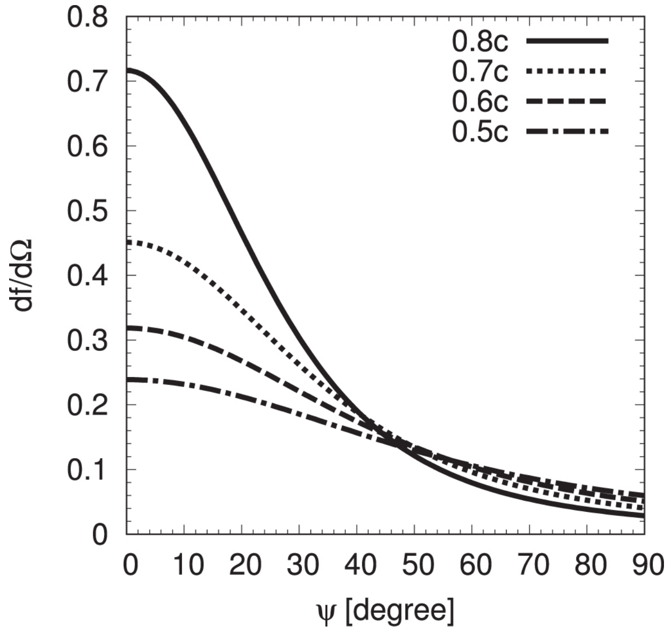
Figure 7. from X-Ray Light Curve and Spectra of Shock Breakout in a Wind null 2018 APJ 853 52 doi:10.3847/1538-4357/aaa482 https://dx.doi.org/10.3847/1538-4357/aaa482 © 2018. The American Astronomical Society. All rights reserved.
