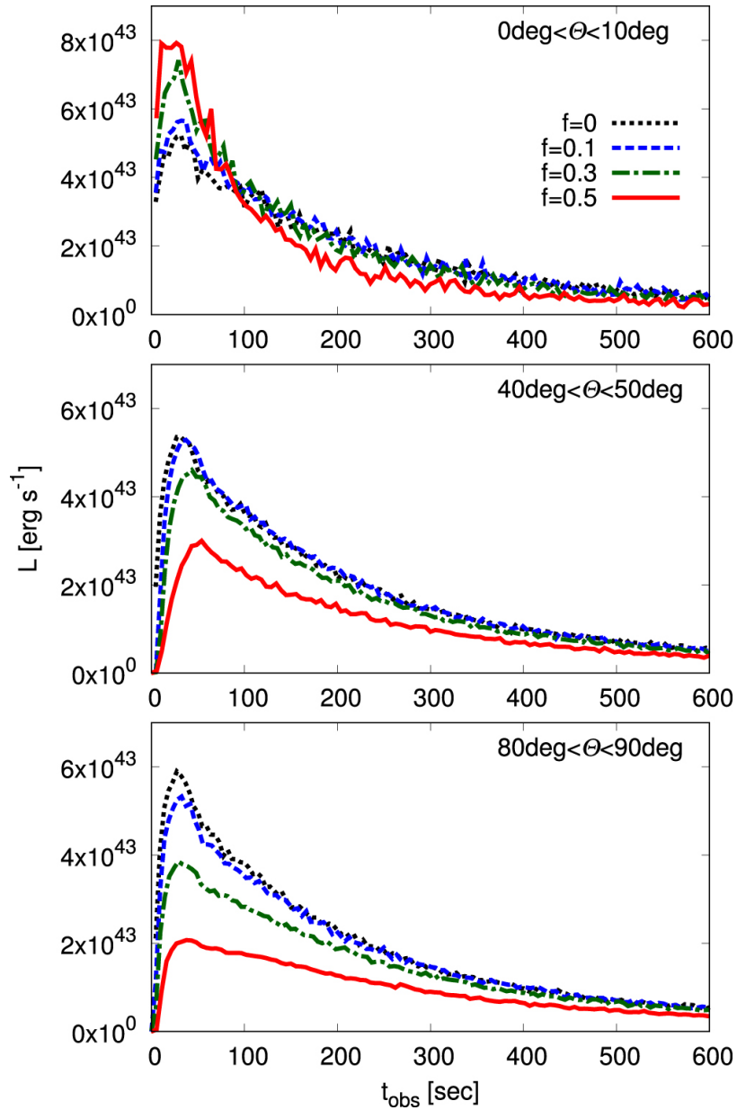
Figure 6. from X-Ray Light Curve and Spectra of Shock Breakout in a Wind null 2018 APJ 853 52 doi:10.3847/1538-4357/aaa482 https://dx.doi.org/10.3847/1538-4357/aaa482 © 2018. The American Astronomical Society. All rights reserved.
