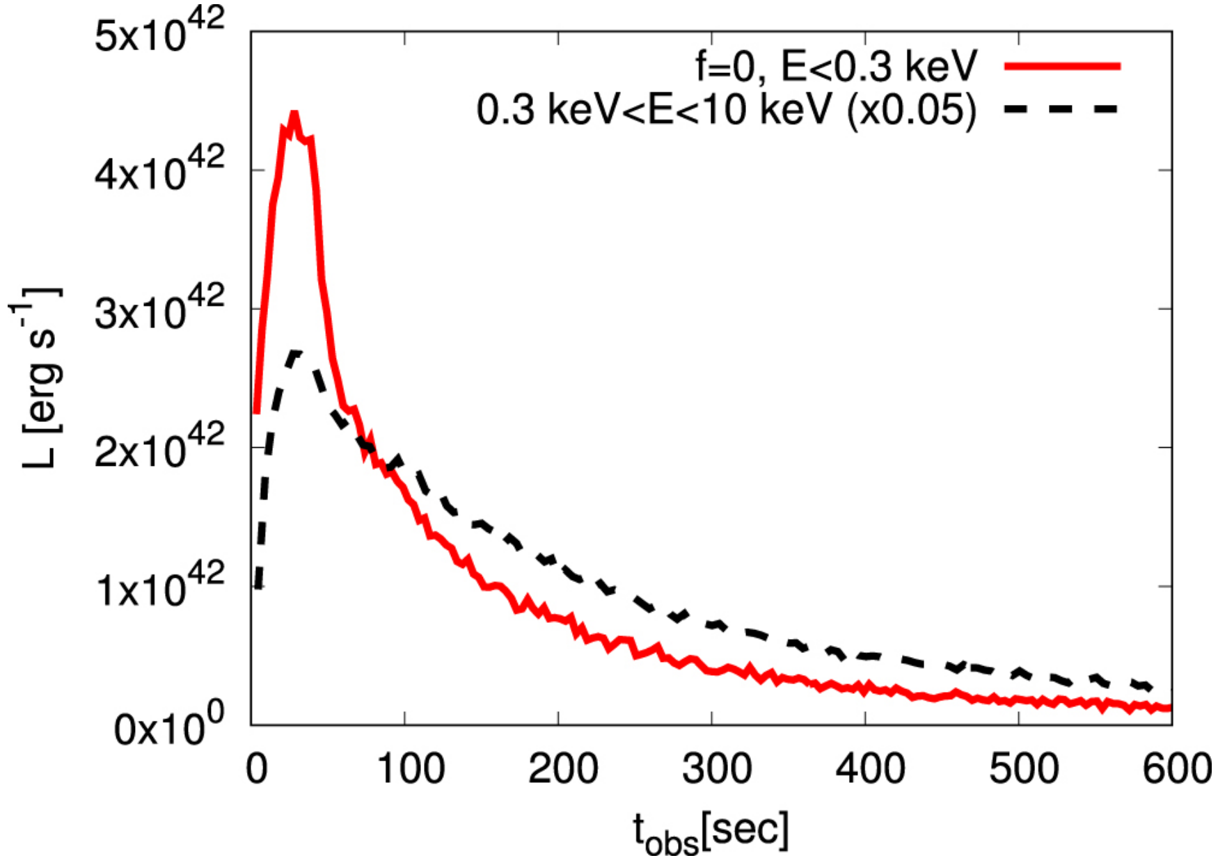
Figure 4. from X-Ray Light Curve and Spectra of Shock Breakout in a Wind null 2018 APJ 853 52 doi:10.3847/1538-4357/aaa482 https://dx.doi.org/10.3847/1538-4357/aaa482 © 2018. The American Astronomical Society. All rights reserved.
