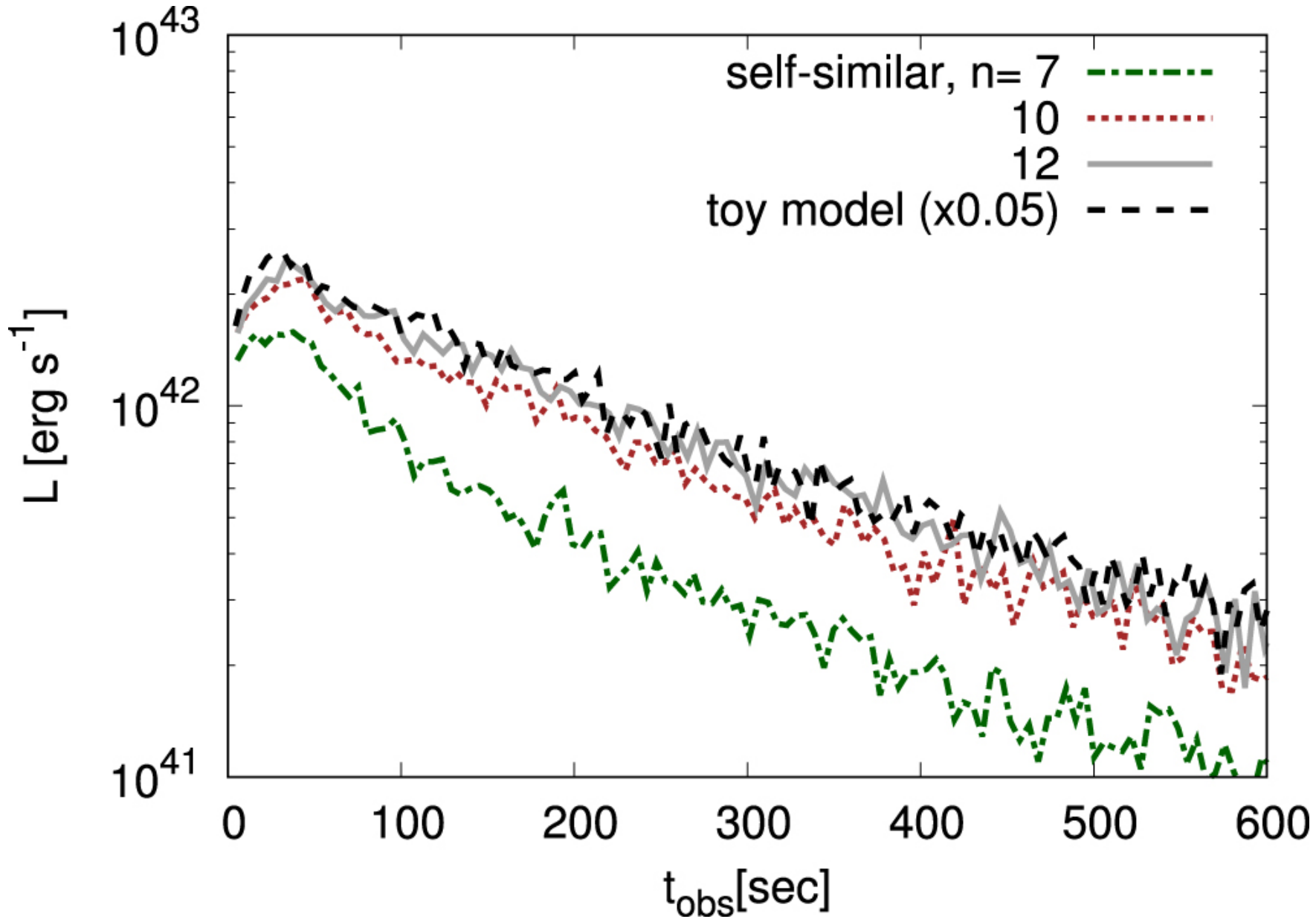
Figure 13. from X-Ray Light Curve and Spectra of Shock Breakout in a Wind null 2018 APJ 853 52 doi:10.3847/1538-4357/aaa482 https://dx.doi.org/10.3847/1538-4357/aaa482 © 2018. The American Astronomical Society. All rights reserved.
