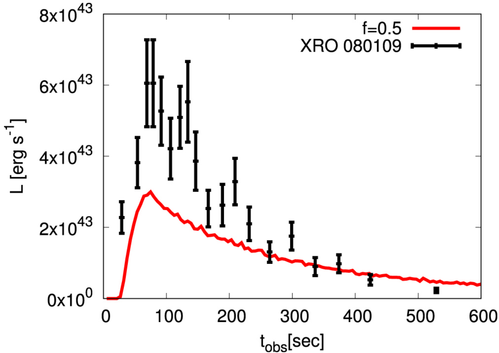
Figure 11. from X-Ray Light Curve and Spectra of Shock Breakout in a Wind null 2018 APJ 853 52 doi:10.3847/1538-4357/aaa482 https://dx.doi.org/10.3847/1538-4357/aaa482 © 2018. The American Astronomical Society. All rights reserved.
