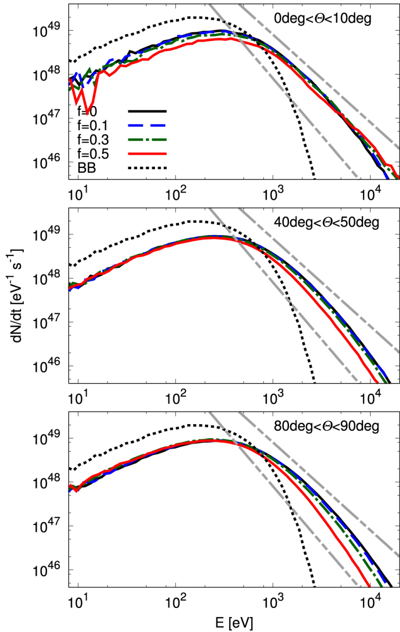
Figure 10. from X-Ray Light Curve and Spectra of Shock Breakout in a Wind null 2018 APJ 853 52 doi:10.3847/1538-4357/aaa482 https://dx.doi.org/10.3847/1538-4357/aaa482 © 2018. The American Astronomical Society. All rights reserved.
