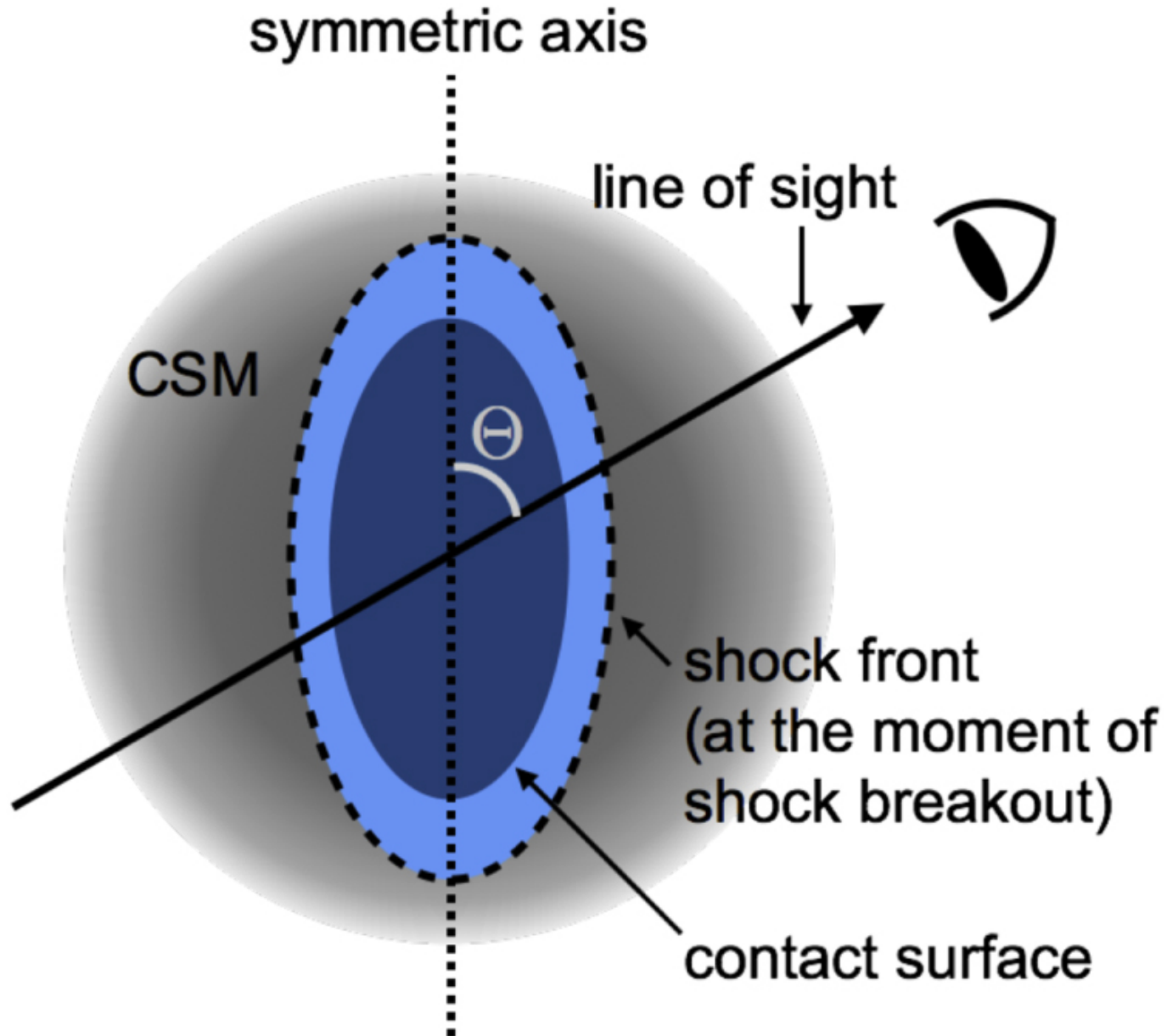
Figure 1. from X-Ray Light Curve and Spectra of Shock Breakout in a Wind null 2018 APJ 853 52 doi:10.3847/1538-4357/aaa482 https://dx.doi.org/10.3847/1538-4357/aaa482 © 2018. The American Astronomical Society. All rights reserved.
