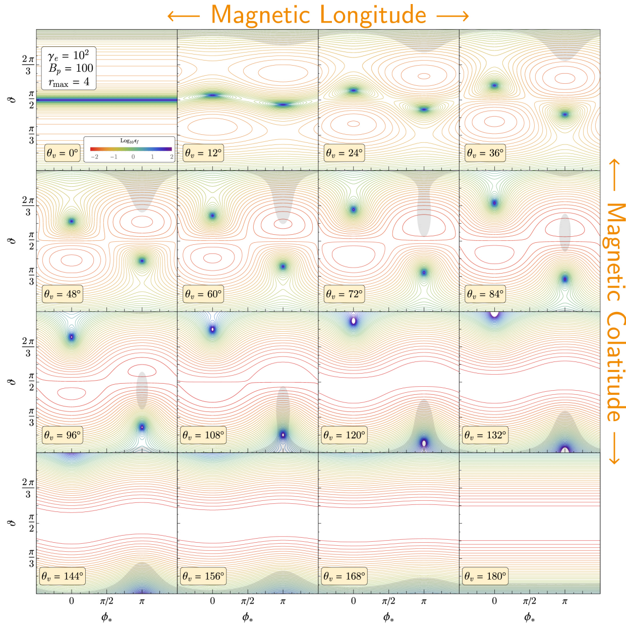
Figure 4. from Resonant Inverse Compton Scattering Spectra from Highly Magnetized Neutron Stars null 2018 APJ 854 98 doi:10.3847/1538-4357/aaa460 https://dx.doi.org/10.3847/1538-4357/aaa460 © 2018. The American Astronomical Society. All rights reserved.
