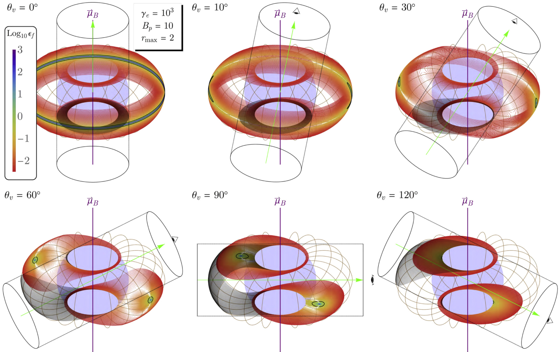
Figure 3. from Resonant Inverse Compton Scattering Spectra from Highly Magnetized Neutron Stars null 2018 APJ 854 98 doi:10.3847/1538-4357/aaa460 https://dx.doi.org/10.3847/1538-4357/aaa460 © 2018. The American Astronomical Society. All rights reserved.
