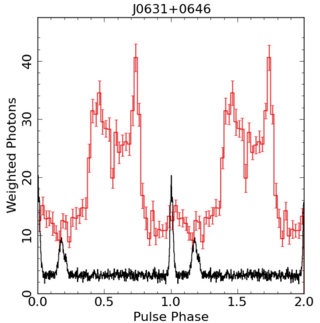
Figure 4. from The Einstein@Home Gamma-ray Pulsar Survey. II. Source Selection, Spectral Analysis, and Multiwavelength Follow-up null 2018 APJ 854 99 doi:10.3847/1538-4357/aaa411 https://dx.doi.org/10.3847/1538-4357/aaa411 © 2018. The American Astronomical Society. All rights reserved.
