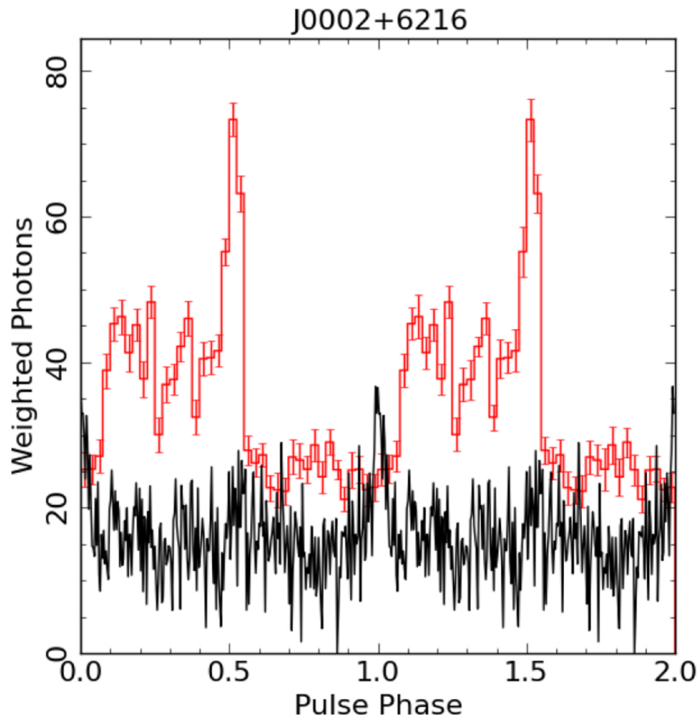
Figure 4. from The Einstein@Home Gamma-ray Pulsar Survey. II. Source Selection, Spectral Analysis, and Multiwavelength Follow-up null 2018 APJ 854 99 doi:10.3847/1538-4357/aaa411 https://dx.doi.org/10.3847/1538-4357/aaa411 © 2018. The American Astronomical Society. All rights reserved.
