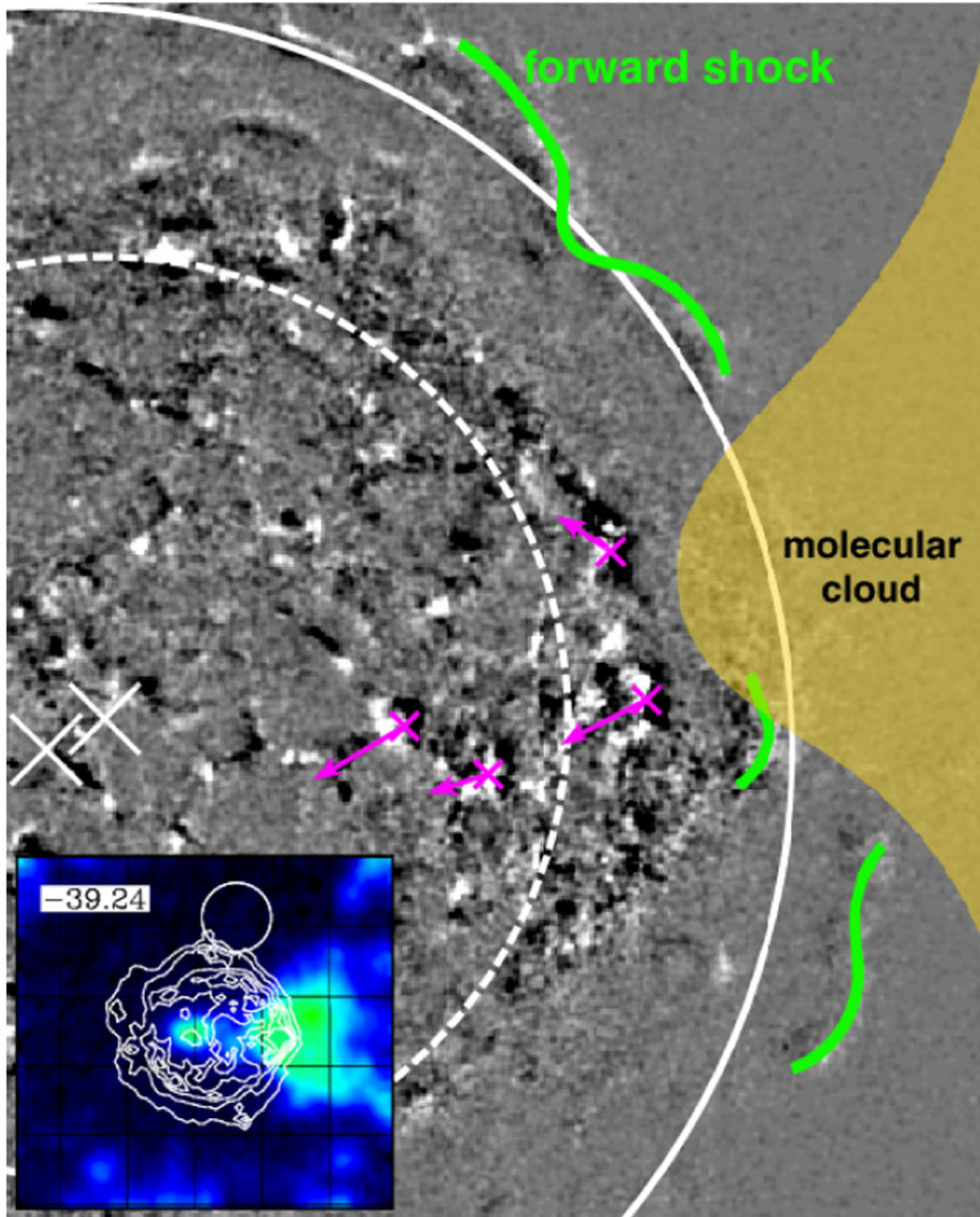
Figure 8. from X-Ray Measurements of the Particle Acceleration Properties at Inward Shocks in Cassiopeia A null 2018 APJ 853 46 doi:10.3847/1538-4357/aaa021 https://dx.doi.org/10.3847/1538-4357/aaa021 © 2018. The American Astronomical Society. All rights reserved.
