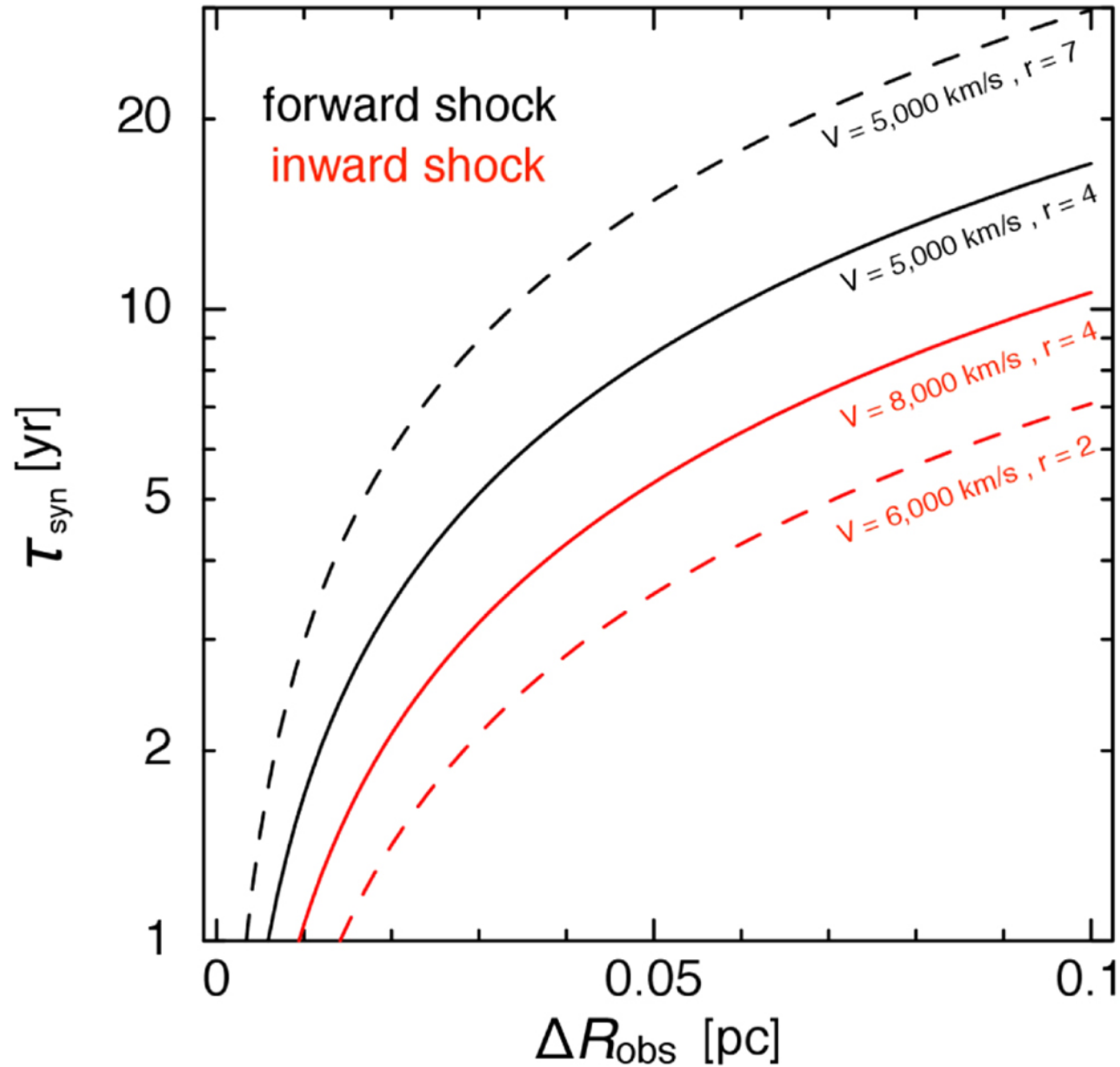
Figure 6. from X-Ray Measurements of the Particle Acceleration Properties at Inward Shocks in Cassiopeia A null 2018 APJ 853 46 doi:10.3847/1538-4357/aaa021 https://dx.doi.org/10.3847/1538-4357/aaa021 © 2018. The American Astronomical Society. All rights reserved.
