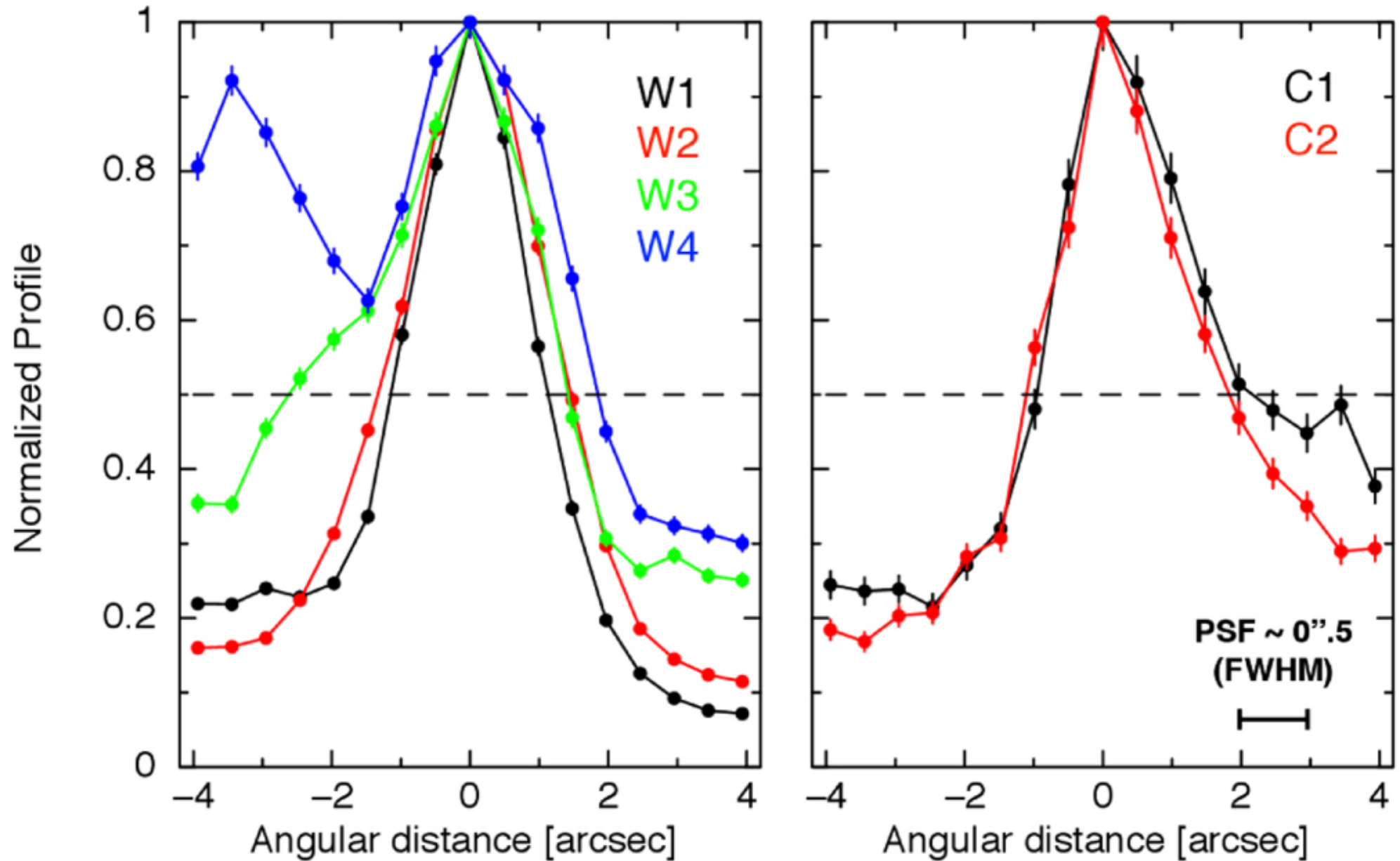
Figure 5. from X-Ray Measurements of the Particle Acceleration Properties at Inward Shocks in Cassiopeia A null 2018 APJ 853 46 doi:10.3847/1538-4357/aaa021 https://dx.doi.org/10.3847/1538-4357/aaa021 © 2018. The American Astronomical Society. All rights reserved.
