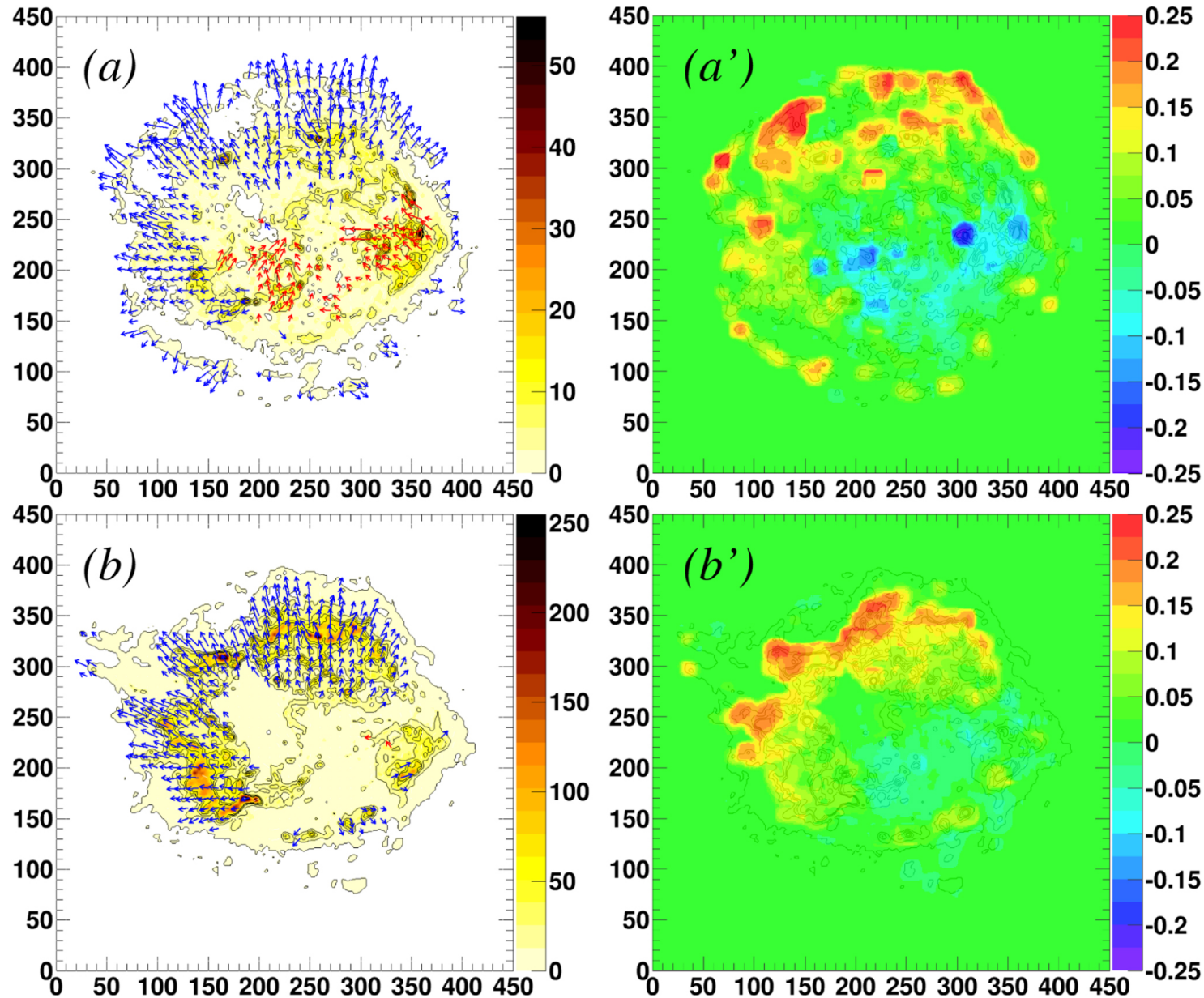
Figure 2. from X-Ray Measurements of the Particle Acceleration Properties at Inward Shocks in Cassiopeia A null 2018 APJ 853 46 doi:10.3847/1538-4357/aaa021 https://dx.doi.org/10.3847/1538-4357/aaa021
