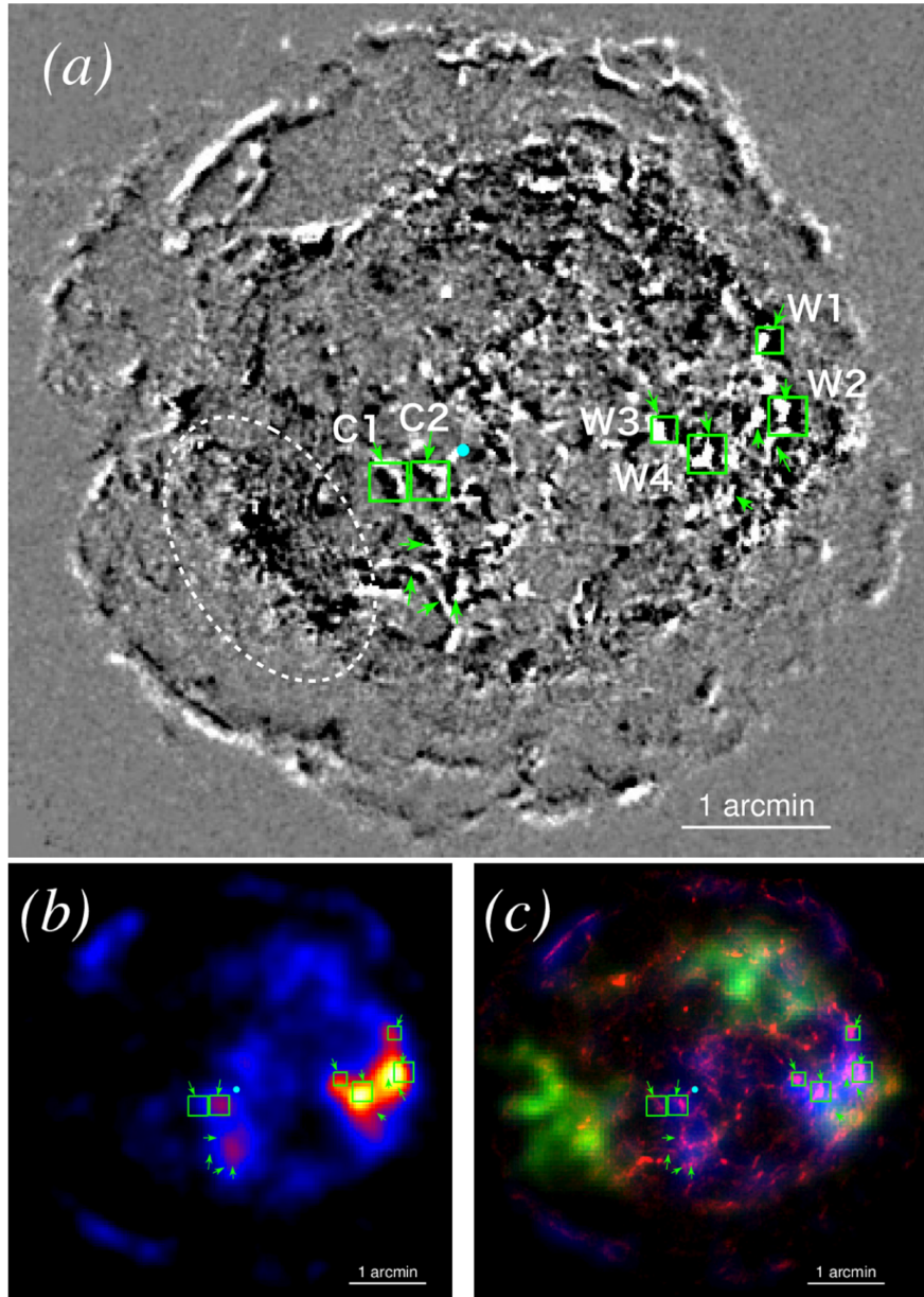
Figure 1. from X-Ray Measurements of the Particle Acceleration Properties at Inward Shocks in Cassiopeia A null 2018 APJ 853 46 doi:10.3847/1538-4357/aaa021 https://dx.doi.org/10.3847/1538-4357/aaa021 © 2018. The American Astronomical Society. All rights reserved.
