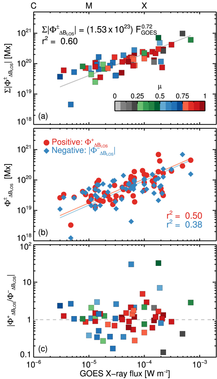
Figure 7. from A Statistical Study of Photospheric Magnetic Field Changes During 75 Solar Flares null 2018 APJ 852 25 doi:10.3847/1538-4357/aa9d37 https://dx.doi.org/10.3847/1538-4357/aa9d37 © 2018. The American Astronomical Society. All rights reserved.
