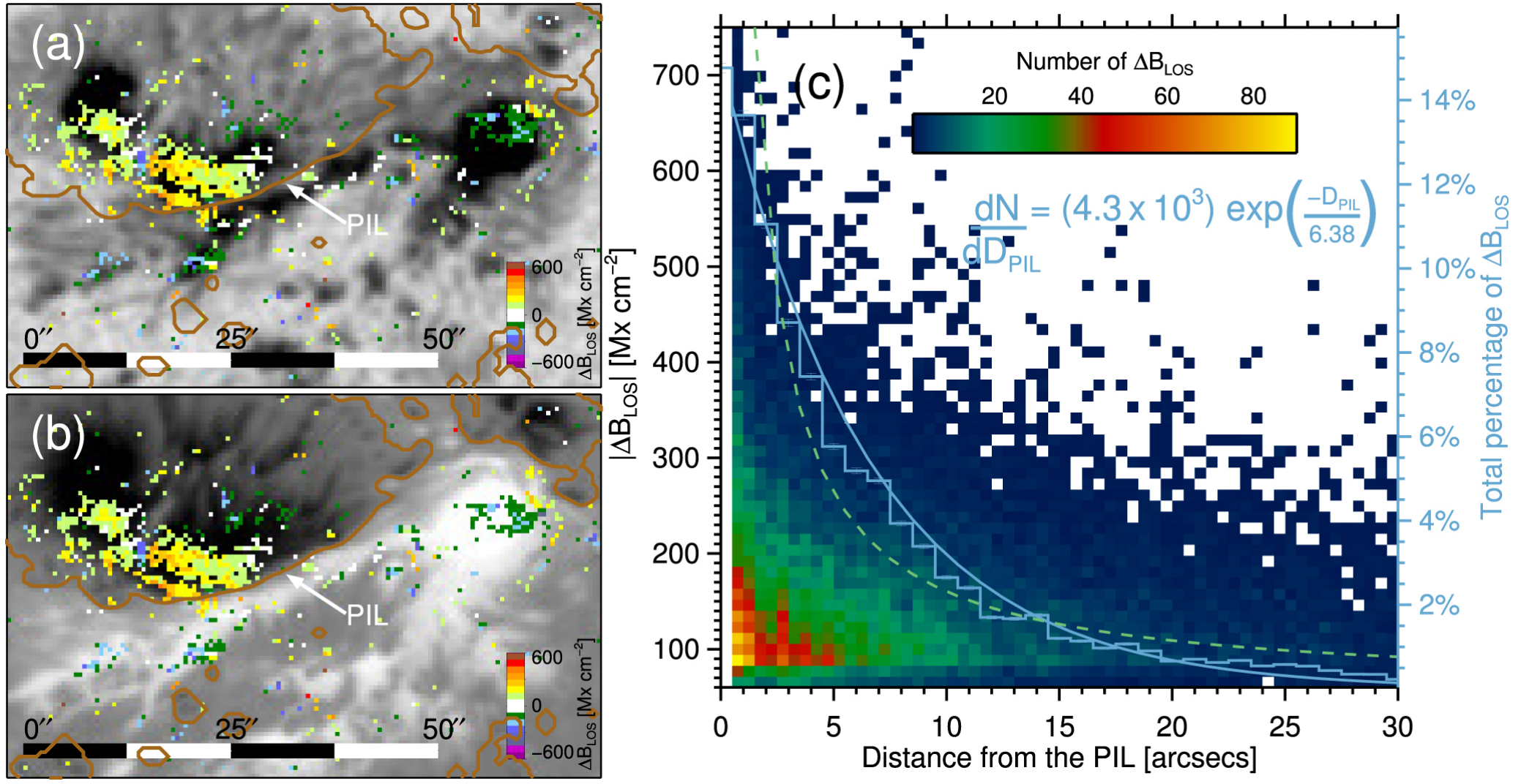
Figure 6. from A Statistical Study of Photospheric Magnetic Field Changes During 75 Solar Flares null 2018 APJ 852 25 doi:10.3847/1538-4357/aa9d37 https://dx.doi.org/10.3847/1538-4357/aa9d37 © 2018. The American Astronomical Society. All rights reserved.
