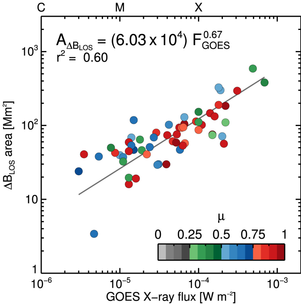
Figure 5. from A Statistical Study of Photospheric Magnetic Field Changes During 75 Solar Flares null 2018 APJ 852 25 doi:10.3847/1538-4357/aa9d37 https://dx.doi.org/10.3847/1538-4357/aa9d37 © 2018. The American Astronomical Society. All rights reserved.
