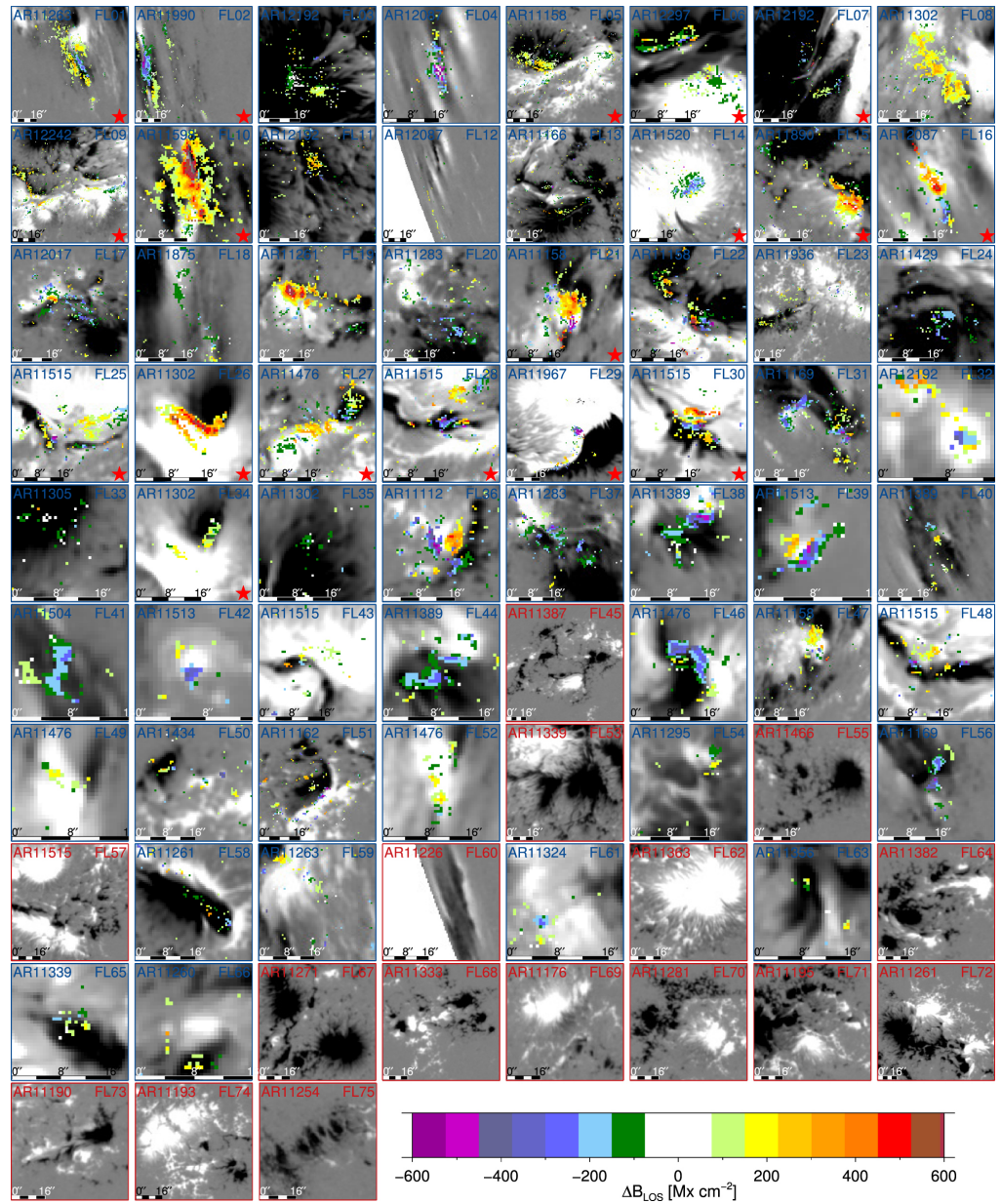
Figure 4. from A Statistical Study of Photospheric Magnetic Field Changes During 75 Solar Flares null 2018 APJ 852 25 doi:10.3847/1538-4357/aa9d37 https://dx.doi.org/10.3847/1538-4357/aa9d37 © 2018. The American Astronomical Society. All rights reserved.
