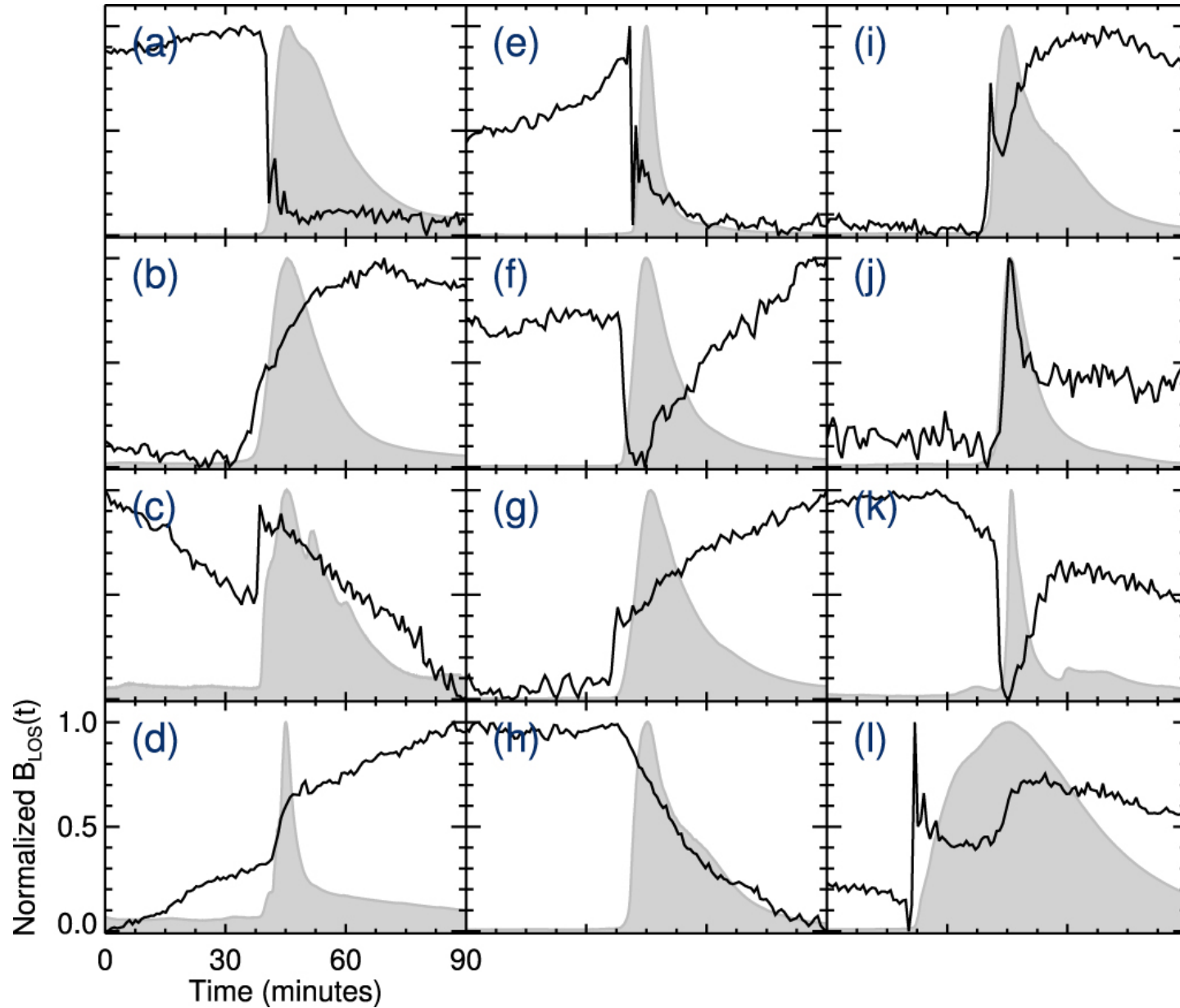
Figure 3. from A Statistical Study of Photospheric Magnetic Field Changes During 75 Solar Flares null 2018 APJ 852 25 doi:10.3847/1538-4357/aa9d37 https://dx.doi.org/10.3847/1538-4357/aa9d37 © 2018. The American Astronomical Society. All rights reserved.
