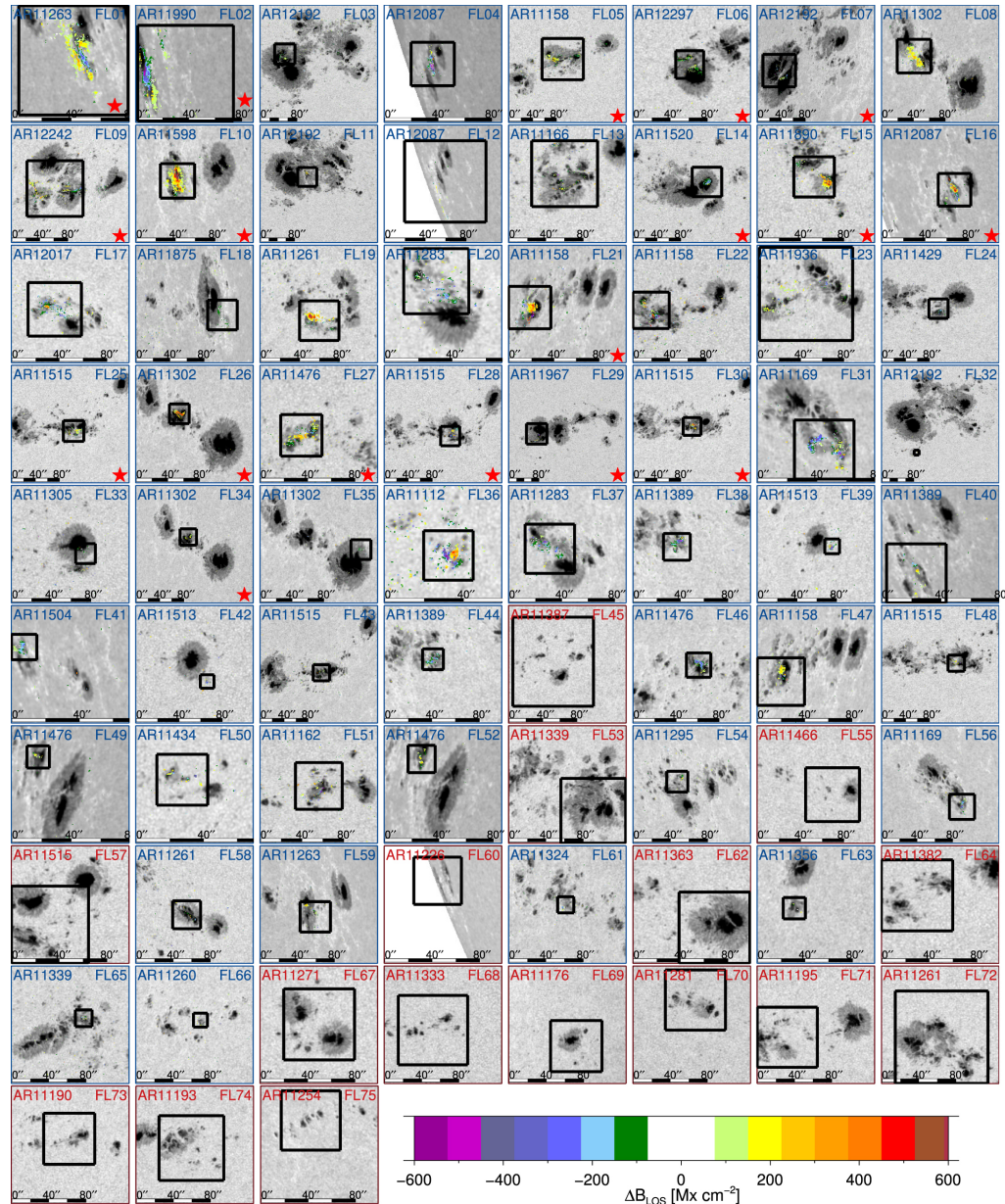
Figure 2. from A Statistical Study of Photospheric Magnetic Field Changes During 75 Solar Flares null 2018 APJ 852 25 doi:10.3847/1538-4357/aa9d37 https://dx.doi.org/10.3847/1538-4357/aa9d37 © 2018. The American Astronomical Society. All rights reserved.
