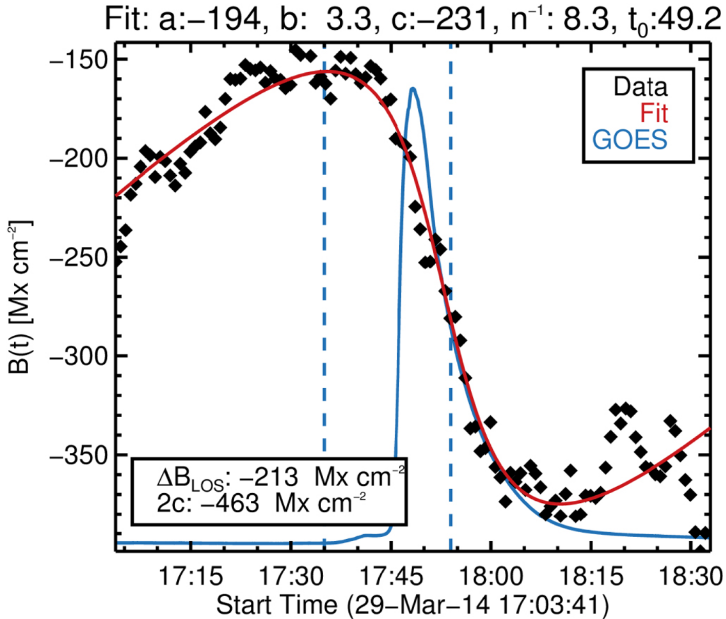
Figure 10. from A Statistical Study of Photospheric Magnetic Field Changes During 75 Solar Flares null 2018 APJ 852 25 doi:10.3847/1538-4357/aa9d37 https://dx.doi.org/10.3847/1538-4357/aa9d37 © 2018. The American Astronomical Society. All rights reserved.
