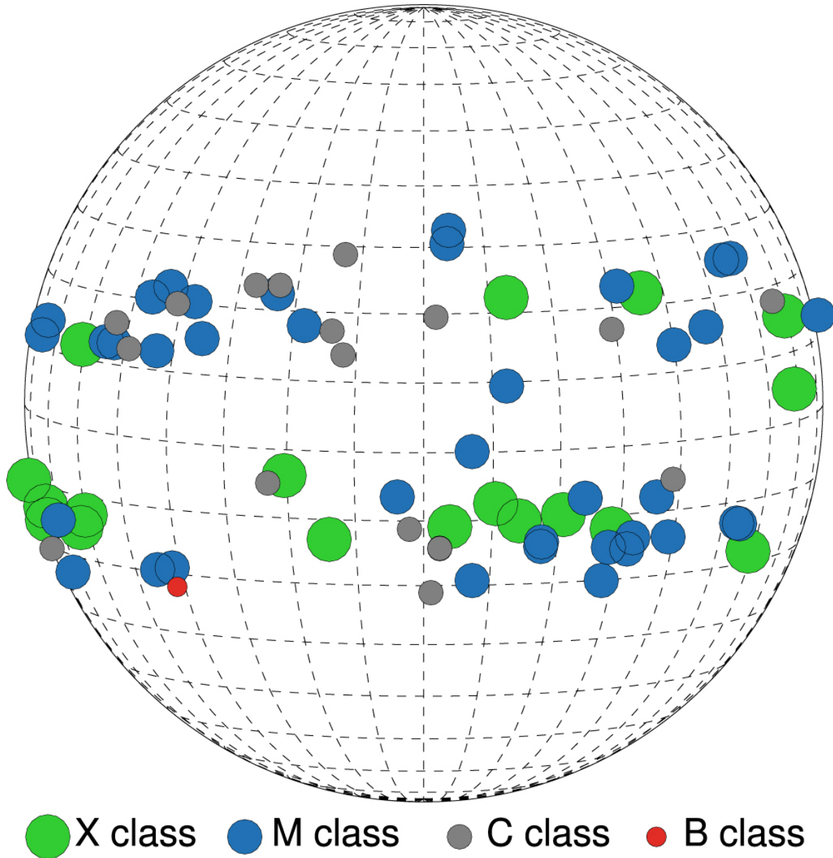
Figure 1. from A Statistical Study of Photospheric Magnetic Field Changes During 75 Solar Flares null 2018 APJ 852 25 doi:10.3847/1538-4357/aa9d37 https://dx.doi.org/10.3847/1538-4357/aa9d37 © 2018. The American Astronomical Society. All rights reserved.
