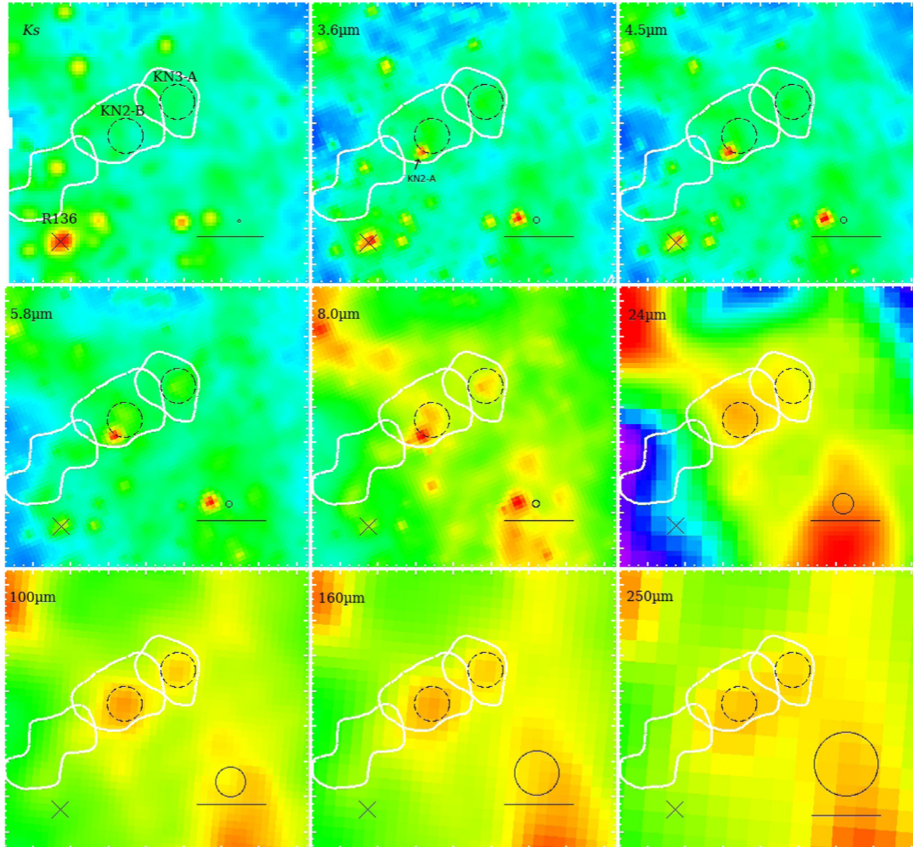
Figure 6. from Pillars of Creation among Destruction: Star Formation in Molecular Clouds near R136 in 30 Doradus null 2018 APJ 852 71 doi:10.3847/1538-4357/aa99dc https://dx.doi.org/10.3847/1538-4357/aa99dc © 2018. The American Astronomical Society. All rights reserved.
