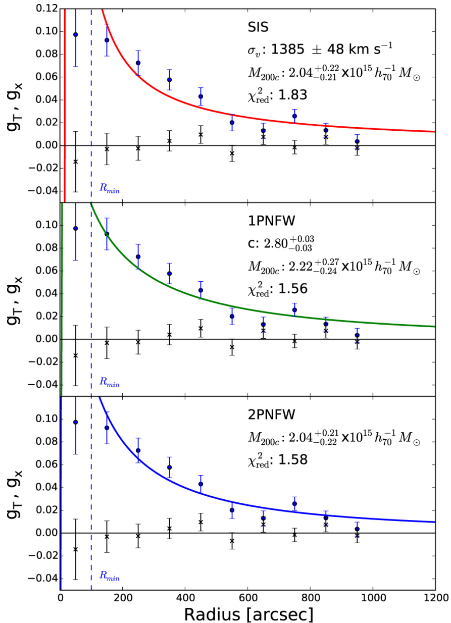
Figure 12. from MC2: Subaru and Hubble Space Telescope Weak-lensing Analysis of the Double Radio Relic Galaxy Cluster PLCK G287.0+32.9 null 2017 APJ 851 46 doi:10.3847/1538-4357/aa998c https://dx.doi.org/10.3847/1538-4357/aa998c
