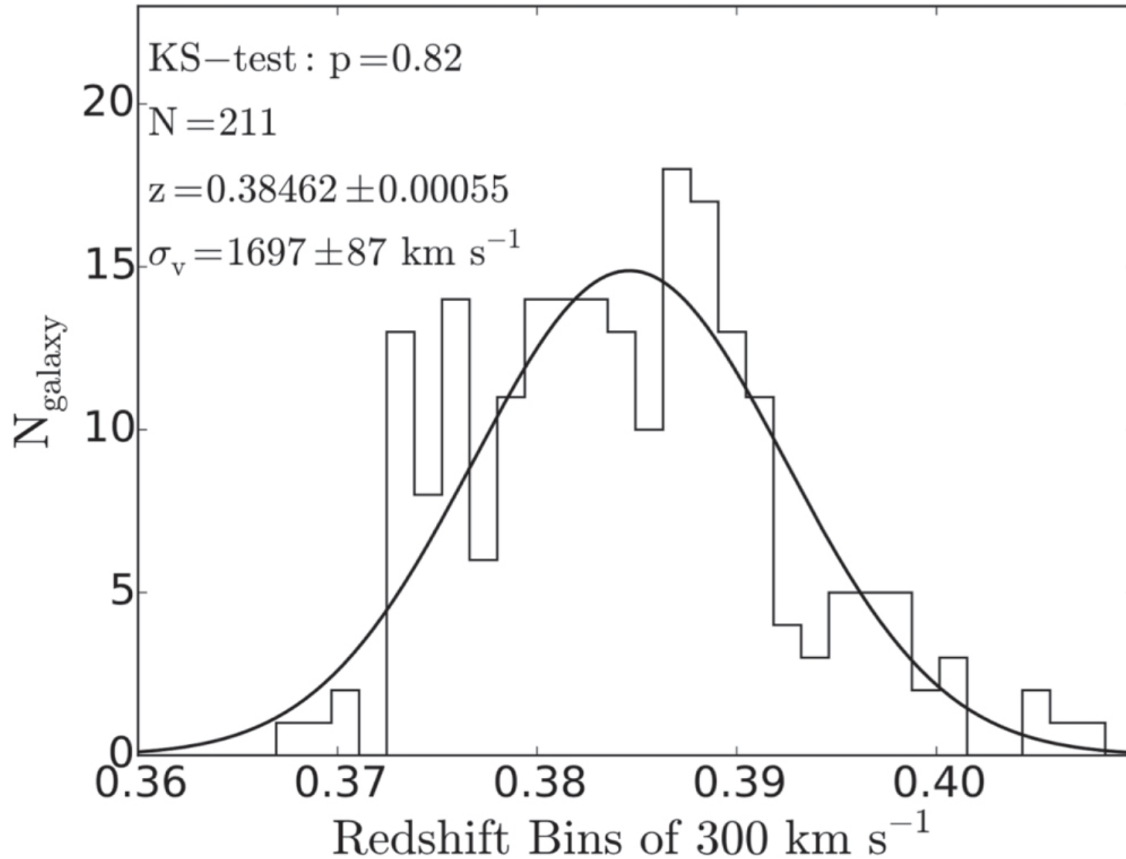
Figure 1. from MC2: Subaru and Hubble Space Telescope Weak-lensing Analysis of the Double Radio Relic Galaxy Cluster PLCK G287.0+32.9 null 2017 APJ 851 46 doi:10.3847/1538-4357/aa998c https://dx.doi.org/10.3847/1538-4357/aa998c © 2017. The American Astronomical Society. All rights reserved.
