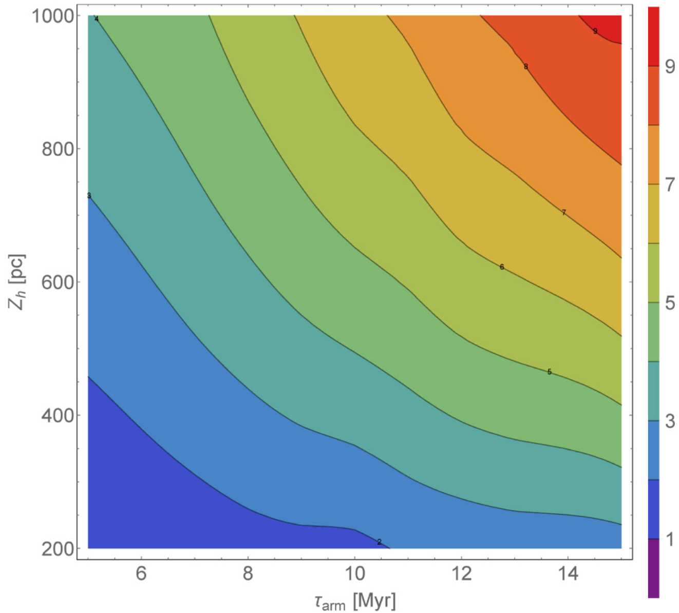
Figure 5. from Electron-capture Isotopes Could Constrain Cosmic-Ray Propagation Models null 2017 APJ 851 109 doi:10.3847/1538-4357/aa9935 https://dx.doi.org/10.3847/1538-4357/aa9935 © 2017. The American Astronomical Society. All rights reserved.
