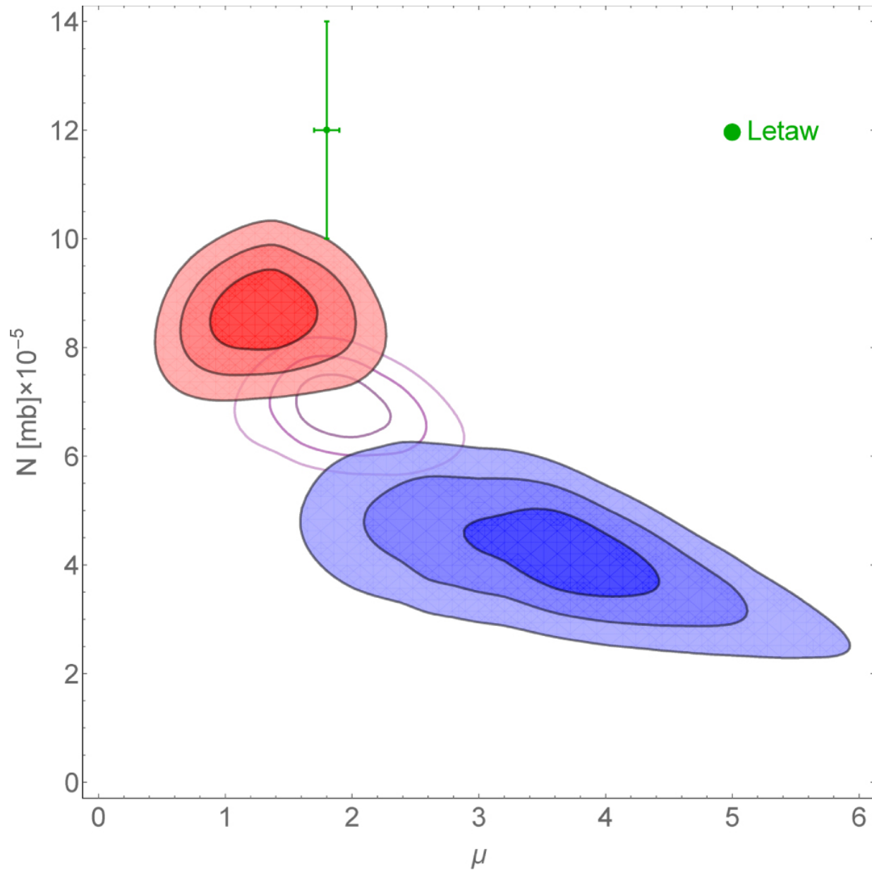
Figure 4. from Electron-capture Isotopes Could Constrain Cosmic-Ray Propagation Models null 2017 APJ 851 109 doi:10.3847/1538-4357/aa9935 https://dx.doi.org/10.3847/1538-4357/aa9935 © 2017. The American Astronomical Society. All rights reserved.
