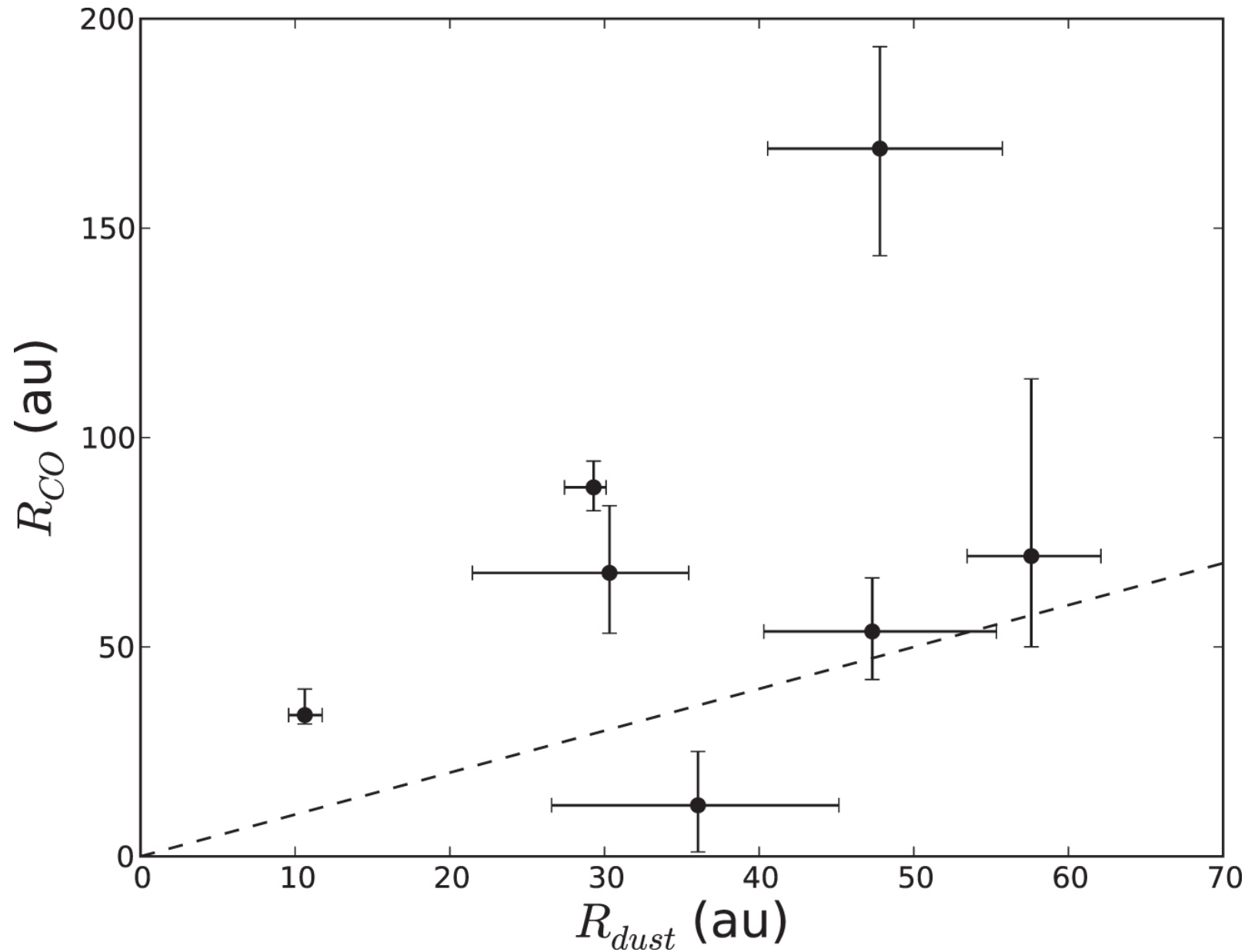
Figure 6. from Measurement of Circumstellar Disk Sizes in the Upper Scorpius OB Association with ALMA null 2017 APJ 851 85 doi:10.3847/1538-4357/aa989d https://dx.doi.org/10.3847/1538-4357/aa989d © 2017. The American Astronomical Society. All rights reserved.
