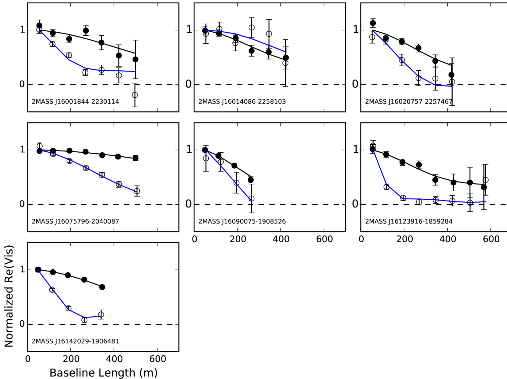
Figure 5. from Measurement of Circumstellar Disk Sizes in the Upper Scorpius OB Association with ALMA null 2017 APJ 851 85 doi:10.3847/1538-4357/aa989d https://dx.doi.org/10.3847/1538-4357/aa989d © 2017. The American Astronomical Society. All rights reserved.
