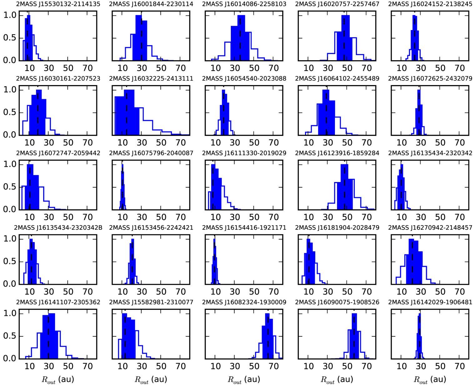
Figure 4. from Measurement of Circumstellar Disk Sizes in the Upper Scorpius OB Association with ALMA null 2017 APJ 851 85 doi:10.3847/1538-4357/aa989d https://dx.doi.org/10.3847/1538-4357/aa989d
