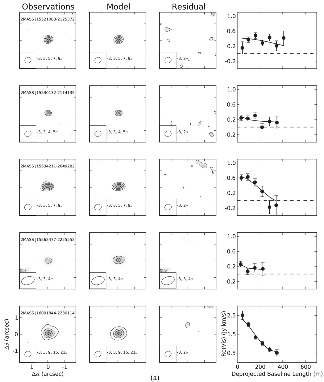
Figure 2. from Measurement of Circumstellar Disk Sizes in the Upper Scorpius OB Association with ALMA null 2017 APJ 851 85 doi:10.3847/1538-4357/aa989d https://dx.doi.org/10.3847/1538-4357/aa989d
