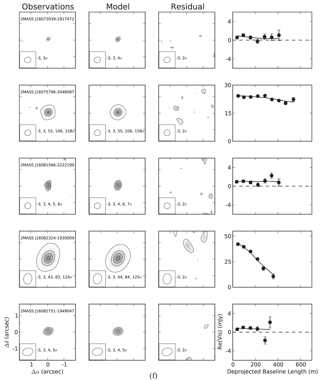
Figure 1. from Measurement of Circumstellar Disk Sizes in the Upper Scorpius OB Association with ALMA null 2017 APJ 851 85 doi:10.3847/1538-4357/aa989d https://dx.doi.org/10.3847/1538-4357/aa989d
