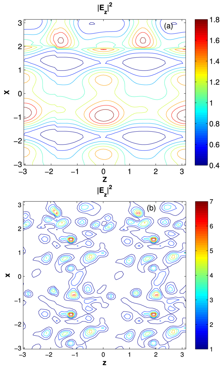
Figure 2. from Quasi-electrostatic Whistler Wave Dynamics in Earth's Radiation Belt null 2017 APJ 851 49 doi:10.3847/1538-4357/aa9716 https://dx.doi.org/10.3847/1538-4357/aa9716 © 2017. The American Astronomical Society. All rights reserved.
