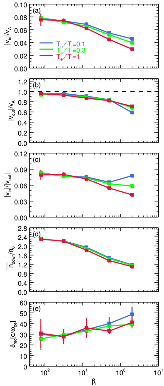
Figure 9. from Electron and Proton Heating in Transrelativistic Magnetic Reconnection null 2017 APJ 850 29 doi:10.3847/1538-4357/aa9380 https://dx.doi.org/10.3847/1538-4357/aa9380 © 2017. The American Astronomical Society. All rights reserved.
