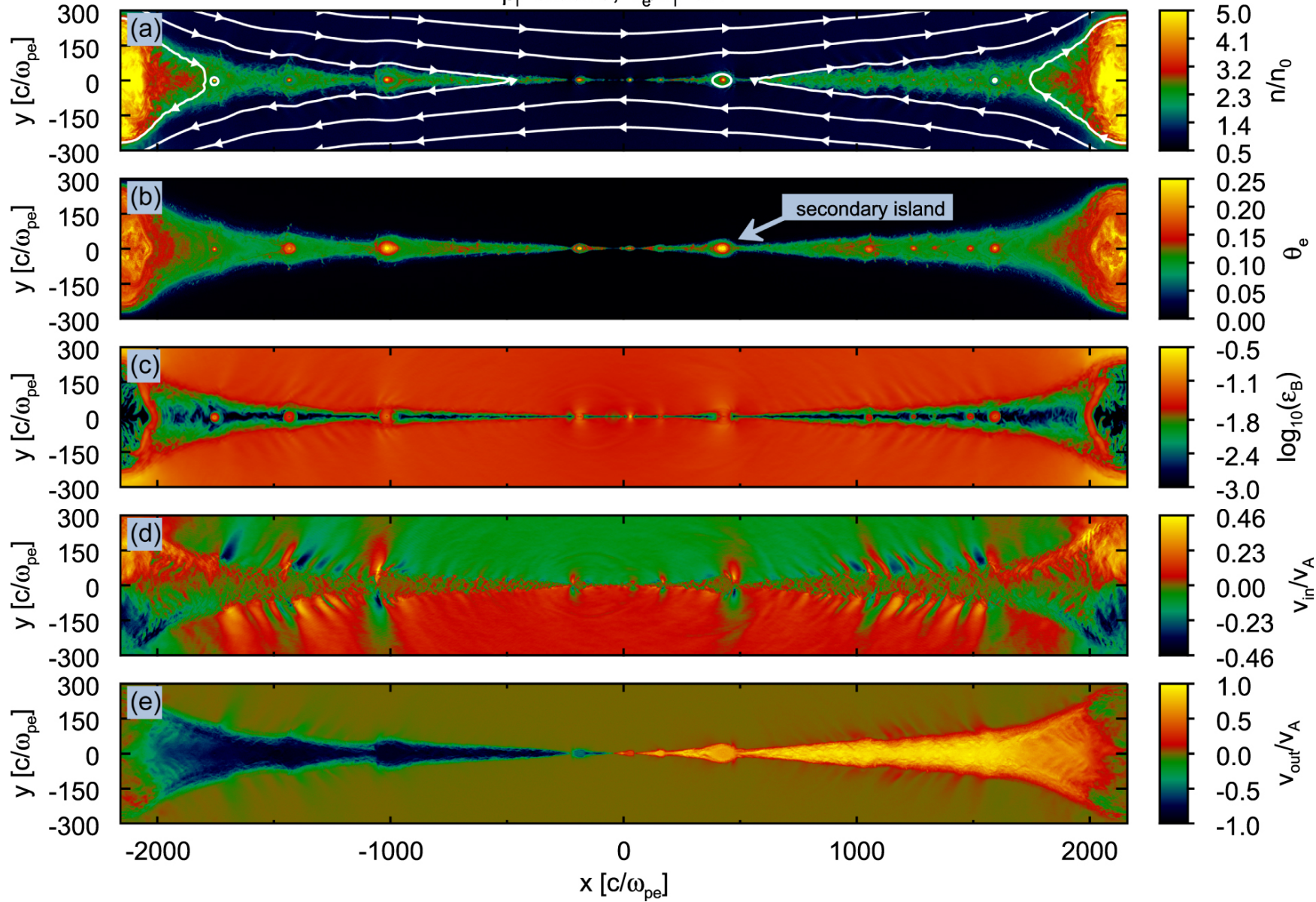
Figure 5. from Electron and Proton Heating in Transrelativistic Magnetic Reconnection null 2017 APJ 850 29 doi:10.3847/1538-4357/aa9380 https://dx.doi.org/10.3847/1538-4357/aa9380 © 2017. The American Astronomical Society. All rights reserved.
