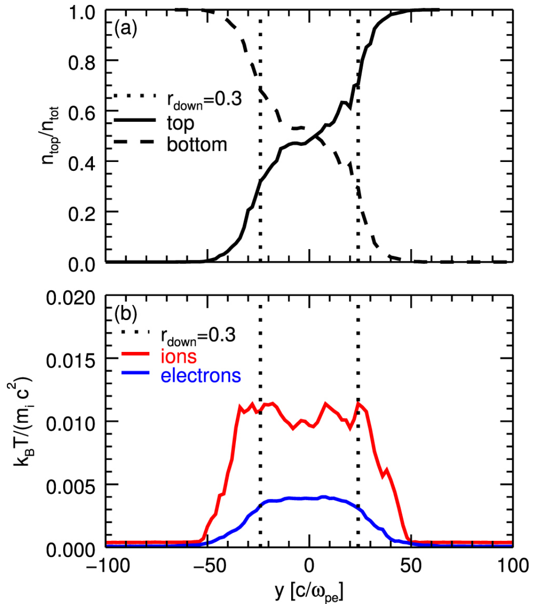
Figure 4. from Electron and Proton Heating in Transrelativistic Magnetic Reconnection null 2017 APJ 850 29 doi:10.3847/1538-4357/aa9380 https://dx.doi.org/10.3847/1538-4357/aa9380 © 2017. The American Astronomical Society. All rights reserved.
