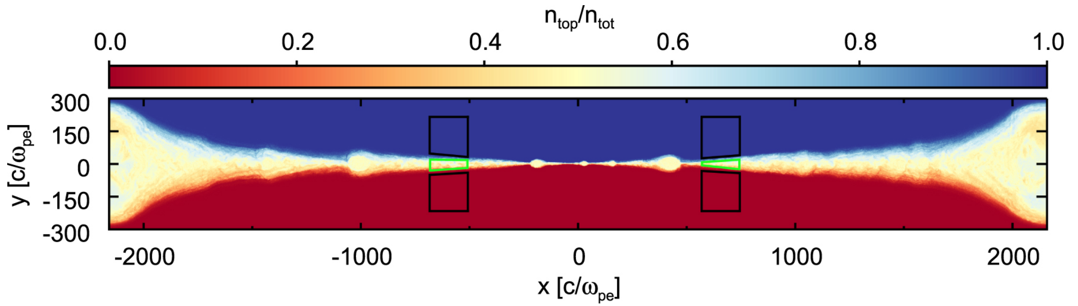
Figure 3. from Electron and Proton Heating in Transrelativistic Magnetic Reconnection null 2017 APJ 850 29 doi:10.3847/1538-4357/aa9380 https://dx.doi.org/10.3847/1538-4357/aa9380 © 2017. The American Astronomical Society. All rights reserved.
